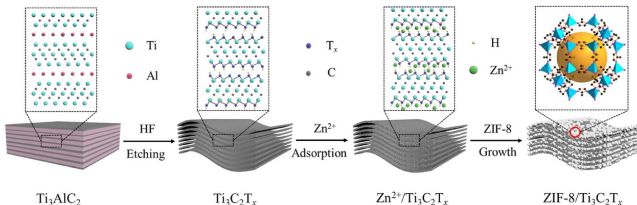
Fig. 3 Illustration of the synthesis of ZIF-8/ \text{Ti}_3\text{C}_2\text{T}_x . Reproduced with permission from ref. 86 Copyright ©2022, Elsevier.
