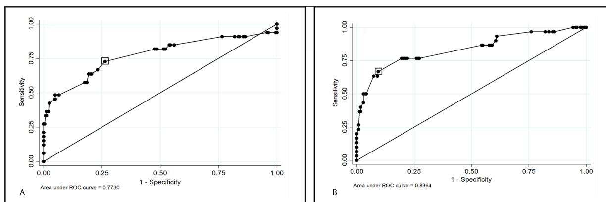
Figure 3: ROC Curves: Use of '+4.00D blur test' to detect significant hyperopia ( \geq+4.00D ). The boxes highlight the best visual acuity cut-off points that relate to the right (sensitivity 72.73%, specificity 73.66%) (A) and left eyes (sensitivity 66.67%, 90.65%) (B).
