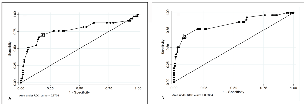
Figure 2: ROC Curves: Use of '+2.50D blur test' to detect significant hyperopia ( \geq+4.00D ). The boxes highlight the best visual acuity cut-off points that relate to the right (sensitivity 69.7%, specificity 81.63%) (A) and left eyes (sensitivity 70.00%, 83.87%) (B).
