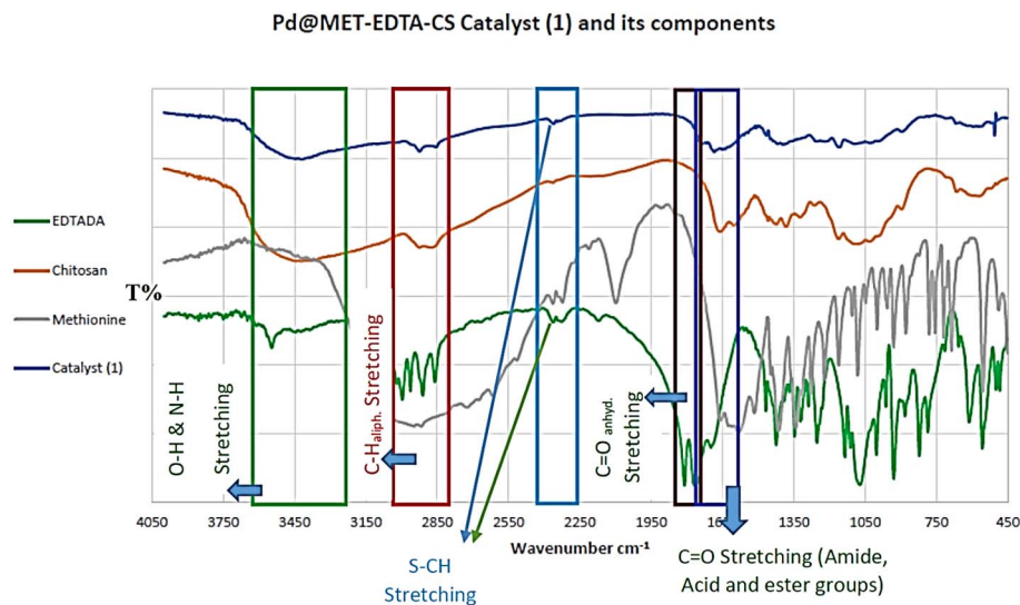
Fig. 1 FTIR spectra of the Pd@MET-EDTA-CS catalyst (1) and its components.
