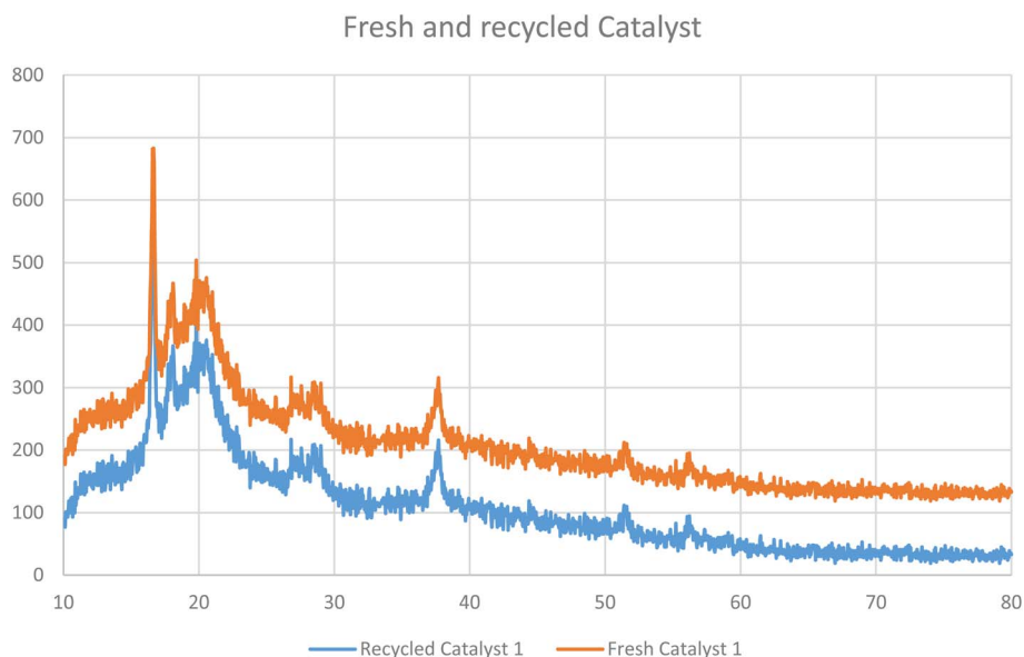
Fig. 13 XRD patterns of the fresh (orange) and recycled (blue) Pd@MET-EDTA-CS nanocatalyst (1).
