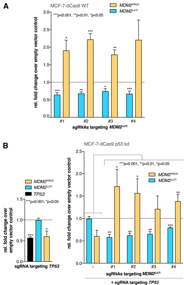
Figure 2 Downregulation of MDM2 LUT1 leads to an increase in the expression of MDM2 PROX in MCF-7 cells, independent of p53 expression. A . RT-qPCR data displaying the changes of MDM2 LUT1 and MDM2 PROX mRNA expression in MCF-7-dCas9 stable cells. The transcription of MDM2 LUT1 was inhibited by CRISPRi using four different sgRNAs (#1-4). Data were normalized to GAPDH , and the fold change relative to the expression of MDM2 LUT1 and MDM2 PROX in the cells transfected with an empty vector was calculated. Data points represent the mean of at least 3 independent biological replicates. Error bars represent standard error of the mean (SEM). Two-tailed Student's t -test was used to calculate the P -values in this figure and all of the subsequent figures. B . RT-qPCR data showing the change in the expression level of TP53 , MDM2 LUT1 and MDM2 PROX in MCF-7-dCas9 cells after CRISPRi-mediated TP53 knockdown (left) or CRISPRi-mediated TP53 - and MDM2 LUT1 -double knockdown (right, sgRNA #1 through #4), relative to the cells transfected with an empty vector. Data were normalized to GAPDH . Data points represent the mean of four biological replicates. Error bars represent SEM.
