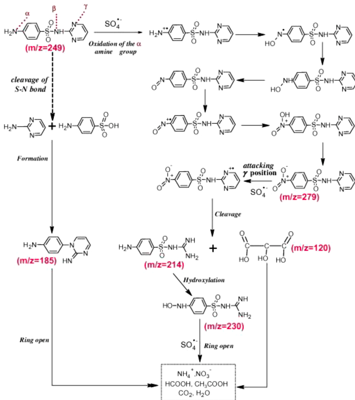
Scheme 5. Proposed SDZ degradation pathways in the sono/Fe 0 /PS system. Reprinted from ref. [75] Copyright (2014), with permission from Elsevier.
