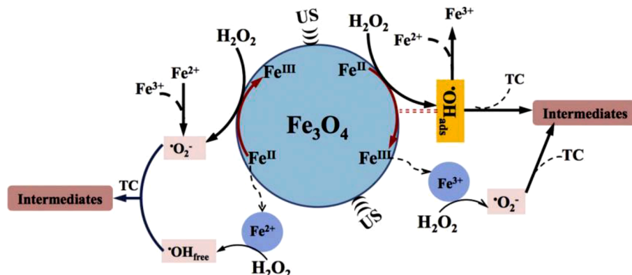
Fig. 3. Mechanism schematic of sono/Fenton-like processes. Reprinted from ref. [32] Copyright (2016), with permission from Elsevier.
