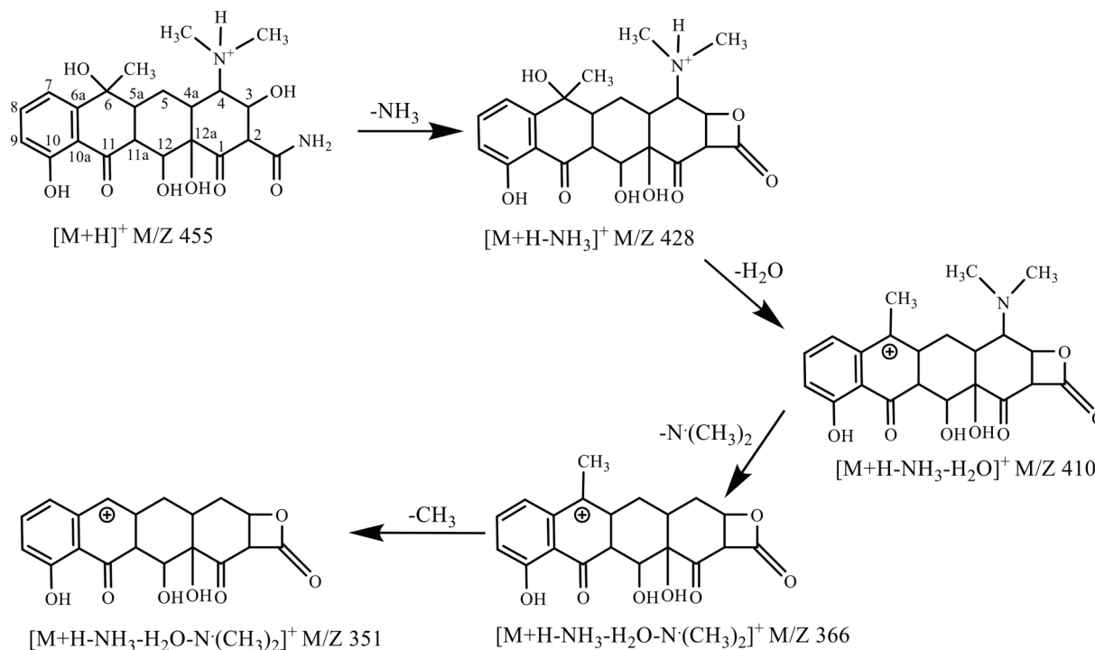
Scheme 3. Proposed degradation pathway for the TC antibiotic in a sono/ \text{S}_2\text{O}_8^{2-} process. Reprinted from ref. [159] Copyright (2017), with permission from Elsevier.
