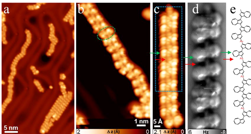
Figure 2. (a) An STM image after annealing 2 on Au(111) at 150 °C ( V_s = -1.5 V, I_t = 0.07 nA) and (b) a close-up STM image of organometallic polymer 3 ( V_s = -0.1 V, I_t = 0.11 nA). A biazulenylyldiyl moiety is marked by a green ellipse. (c) A high-resolution STM image of an organometallic chain imaged by a CO-functionalized tip ( V_s = -0.05 V, I_t = 0.1 nA). (d) A bond-resolved nc-AFM image of the marked region in (c) ( V_s = -5 mV, oscillation amplitude: ~80 pm) and its (e) assigned chemical structure.
