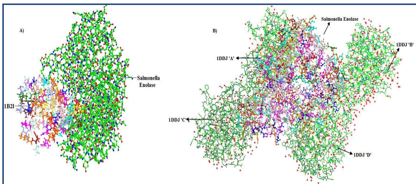
Figure 2: Plasminogen-enolase interaction with 1B2I (A) and 1DDJ (B) domains respectively
