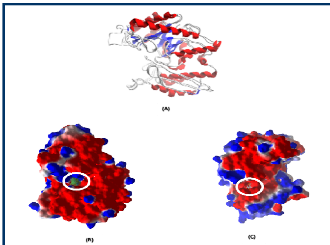
Figure 1: Salmonella and human enolase overlapping complex (A), docked regions being highlighted in circles in Human (B) and Salmonella (C) enolase respectively
