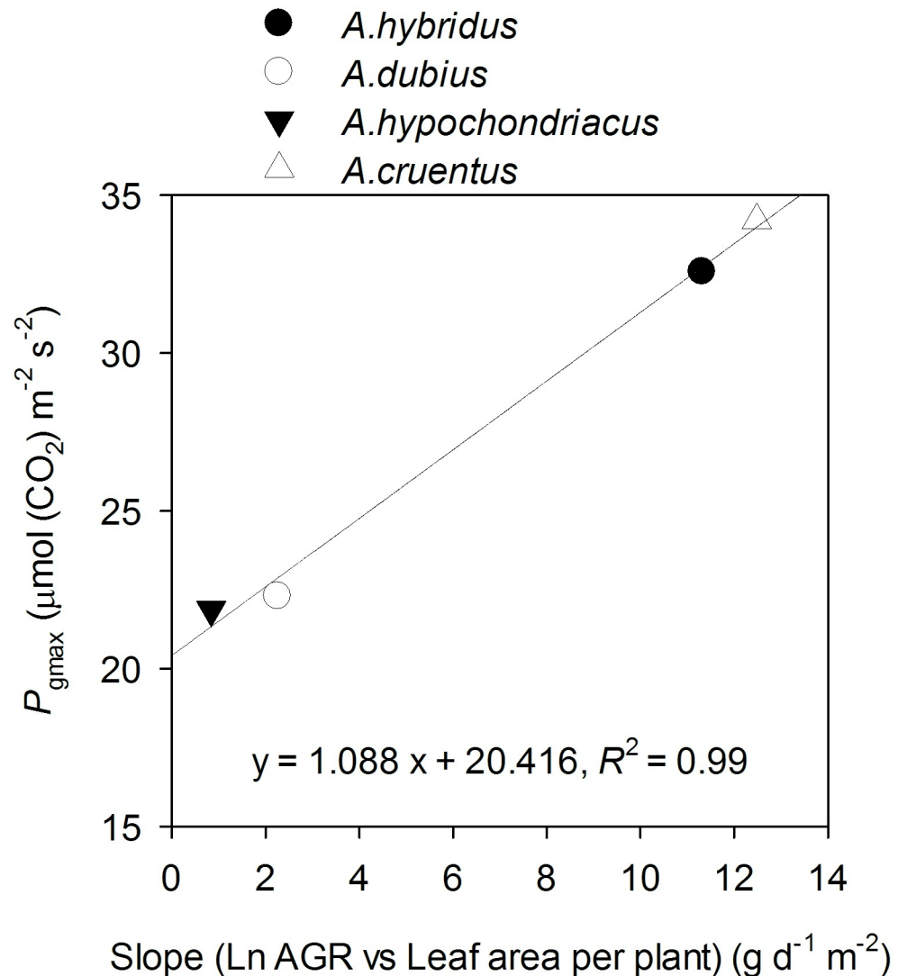
Fig 6. The relationship between maximum gross photosynthetic rate ( P_{\text{gmax}} ) and the slope between the natural logarithm of absolute growth rate and leaf area per plant.
