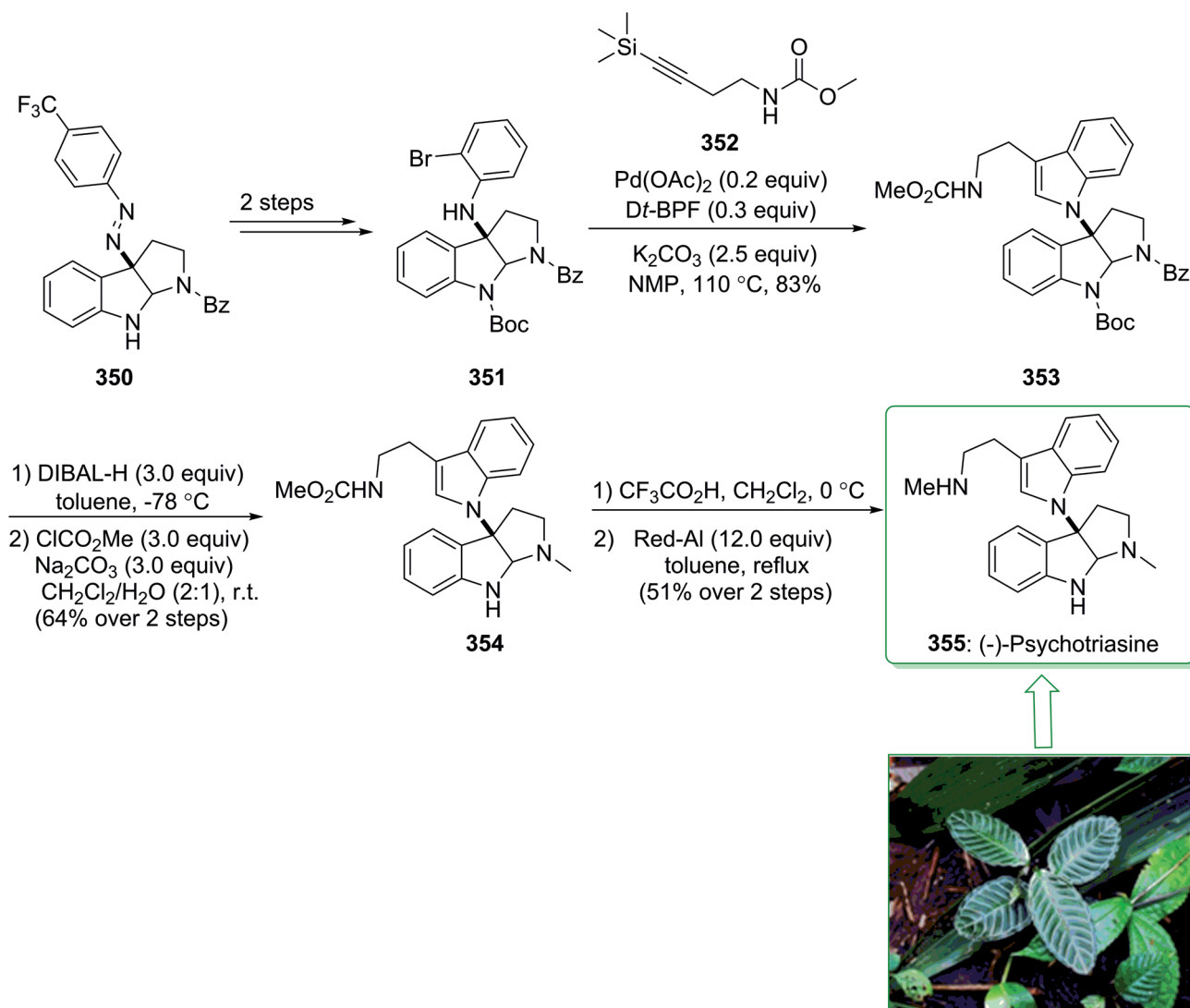
Scheme 48 Asymmetric total synthesis of (-)-psychotriasine ( 355 ).
