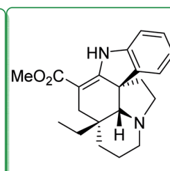
136 : (+)-Vincadifformine
