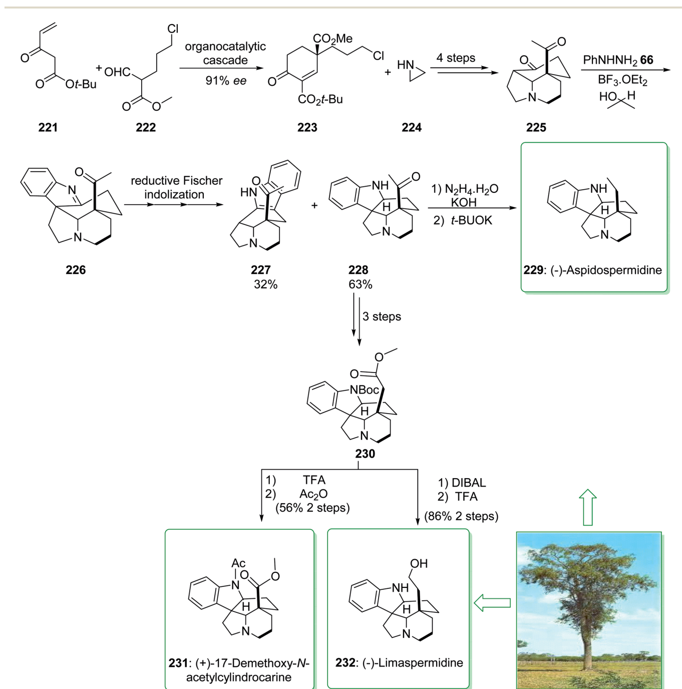
Scheme 29 Total synthesis of (–)-aspidospermidine ( 229 ), (+)-17-demethoxy- N -acetylcylindrocarine ( 231 ) and (–)-limaspermidine ( 232 ).
