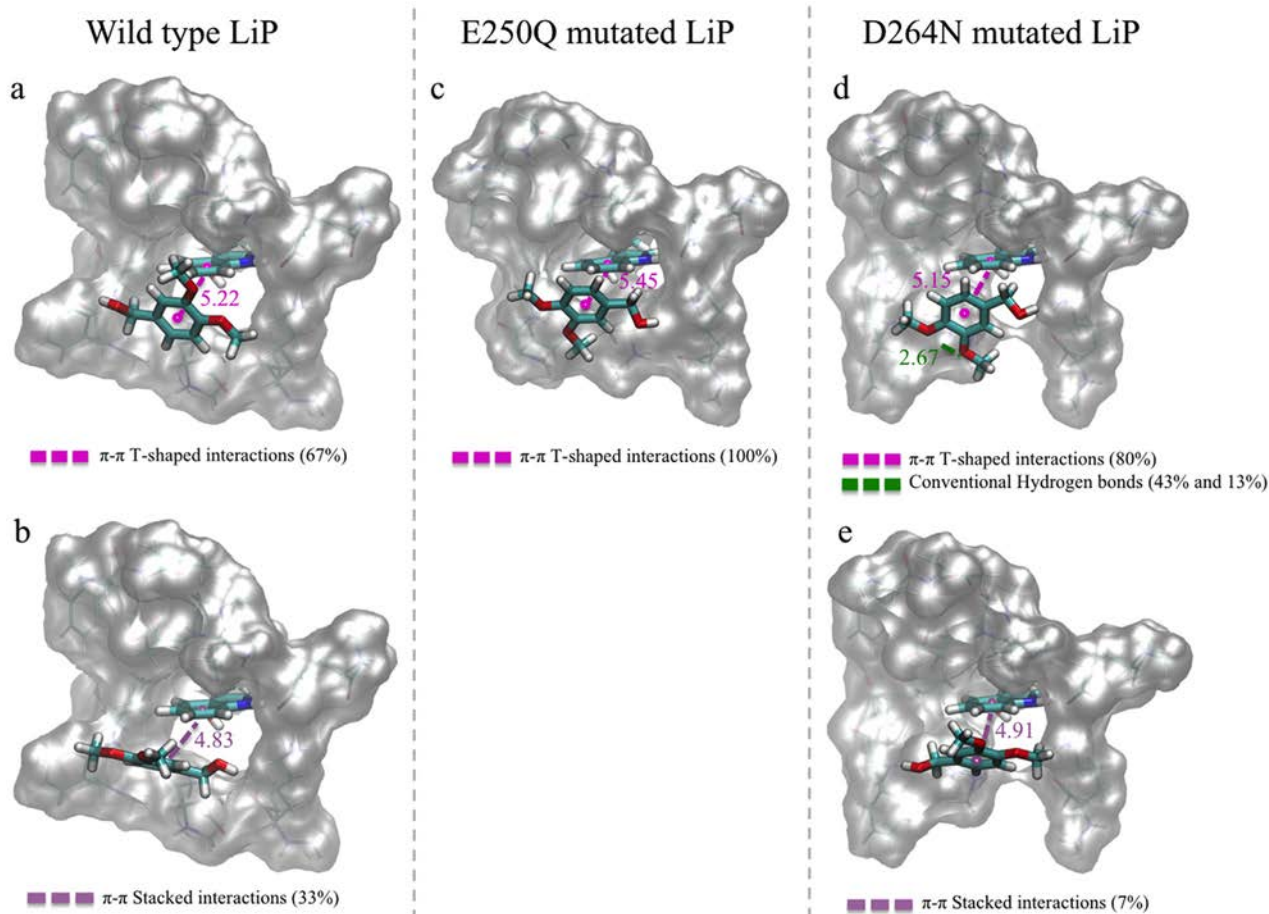
Fig. 2. Main \pi - \pi stacking intermolecular interactions in the LiPH8 Trp171-VA + complexes with the best interaction energies, corresponding to: (a,b) wild-type LiP region, (c) E250Q variant region, and (d, e) D264N variant region.
