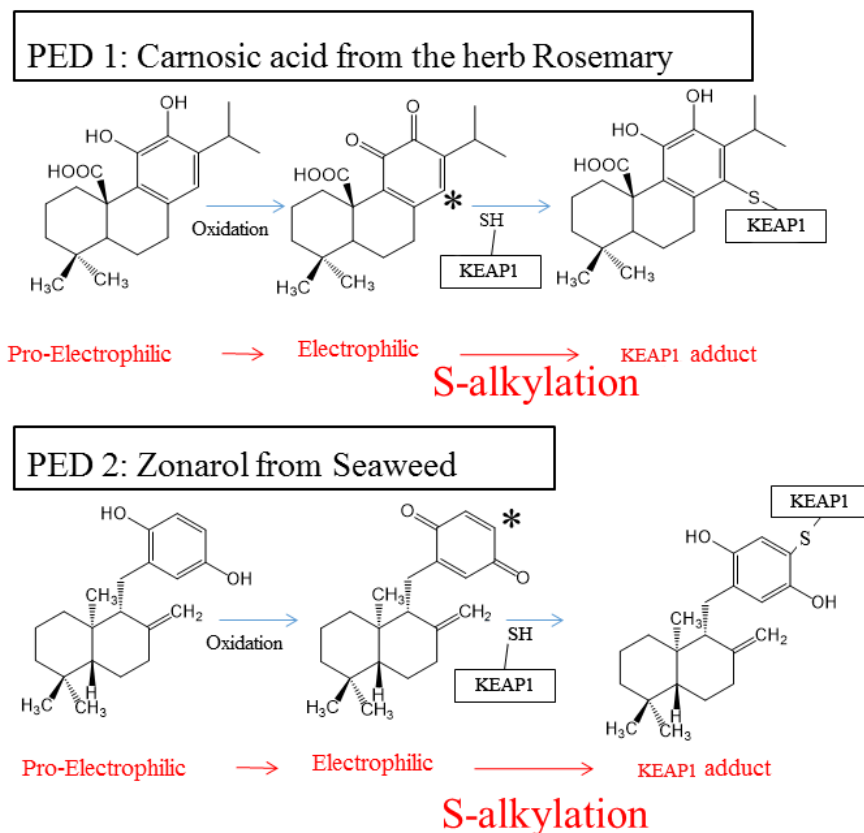
Figure 3. Activation of the KEAP1/NRF2 pathway by PEDs (PED 1, CA; PED 2, ZO). The PED compounds CA (with adjacent or “ ortho ” position hydroxyl groups) 46,47,49,50 and ZO (with hydroxyl groups located directly across the ring, in the “ para ” position) 51,52 become oxidized to the electrophilic quinone form. CA and ZO quinones undergo nucleophilic attack by a critical KEAP1 cysteine thiol. The reaction forms a KEAP1-CA or KEAP1-ZO adduct. This results in release of NRF2 from KEAP1/NRF2 complexes, accumulation of NRF2 in the nucleus, and subsequent transcriptional activation of phase II enzymes 45,46 . Phase II anti-oxidant and anti-inflammatory enzymes reduce reactive oxygen species and thus improve the resilience of neurons. Importantly, the oxidation of hydroquinone (PED) to quinone (EP) is triggered by oxidative stress, which is then combatted by this transcriptional activity, as described in the text 45,49 . CA, carnosic acid; EP, electrophile; KEAP1, Kelch-like ECH-associated protein 1; NRF2, nuclear factor erythroid 2-related factor 2; PD, Parkinson's disease; PED, pro-electrophilic drug; ZO, zonarol.
