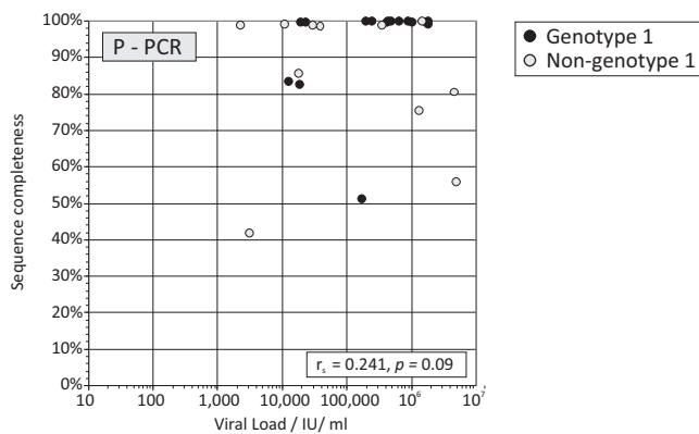
FIG 2 Relationship between viral load and completeness of the HCV consensus sequence from each method. (A to C) The proportion of the whole genome sequenced was compared with viral loads separately for target enrichment (A), metagenomics (B), and sequence preamplified by PCR (C) (plotted on a common x/y scale). Sequence completeness was expressed as a percentage, assuming a genome length of 9,650 bases. Genotype 1 and non-genotype 1 samples are indicated according to the symbol key. The significance of the association between viral load and genome coverage was calculated by Spearman's rank order correlation test; values of r_s and P values are provided in inset boxes.
