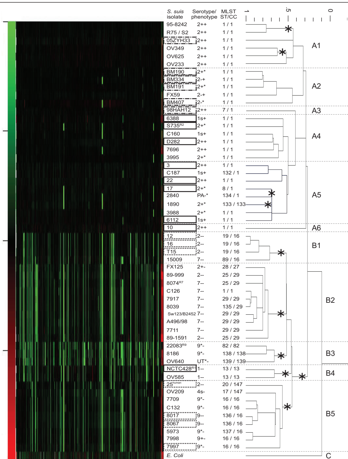
Figure 1 Dendrogram of normalized CGH results. S. suis strains are listed in the first column, serotype and phenotype (muramidase released protein (MRP) and extracellular factor (EF) expression) in the second column. MLST sequence type (ST) and clonal complex (CC) are listed in the last column. Red color indicates probes that are present in more copies than in P1/7, whereas green color indicates probes that are present in P1/7, and absent in the test strain. Asterisks indicate statistically significant knots. Solid boxed isolates were shown to be virulent or weakly virulent in experimental infections; dotted boxed isolates were shown to be avirulent or very weakly virulent in experimental infections; striped - dotted boxed isolates were isolates from human patients. human indicates an isolate that was shown to be avirulent in experimental infection, but was isolated from a human patient.
