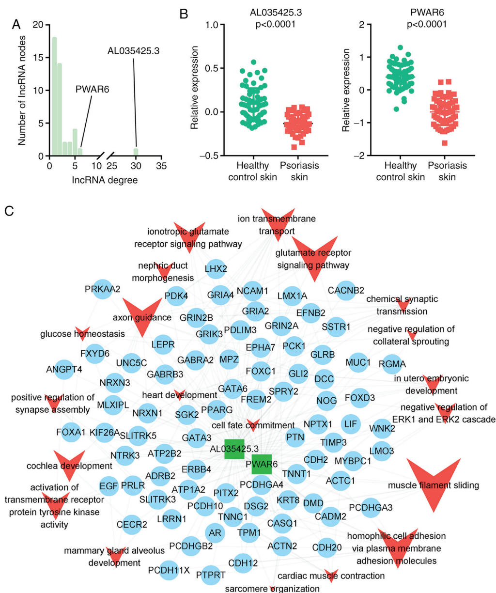
Figure 5. Identification of key lncRNA analysis. (A) The degree distribution of lncRNAs in the downregulated lncRNA-mediated ceRNA network are presented. (B) Expression level of two key lncRNAs in psoriasis skin and healthy control skin. (C) Key downregulated lncRNA-mediated biological processes analysis. lncRNA, long non-coding RNA; ceRNA, competing endogenous RNA; PWAR6, Prader Willi/Angelman region RNA 6.
