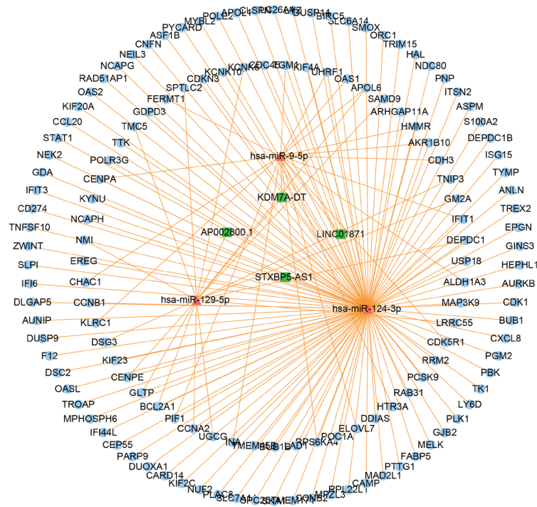
Figure 3. Construction of upregulated lncRNA-mediated ceRNA network. Green nodes, lncRNAs; red nodes, miRNAs; blue nodes, mRNAs. lncRNA, long non-coding RNA; miR/miRNA, microRNA; hsa, Homo sapiens .
