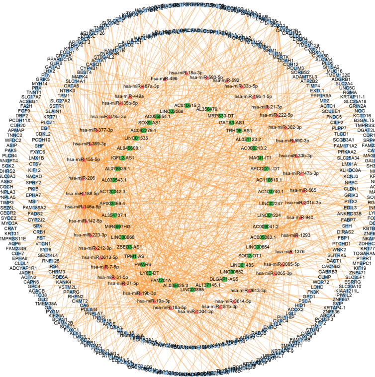
Figure 4. Construction of downregulated lncRNA-mediated ceRNA network. Green nodes, lncRNAs; red nodes, miRNAs; blue nodes, mRNAs. lncRNA, long non-coding RNA; miR/miRNA, microRNA; hsa, Homo sapiens .
