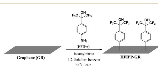
Fig. 1 Preparation of p -hexafluoroisopropanol phenyl functionalized graphene.
