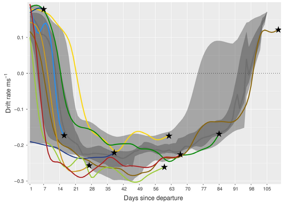
FIGURE 8 Drift rates of non-survivors (colors correspond to individuals), with times of death (and corresponding drift rates) indicated by black stars. The large light gray band represents the 2.5%–97.5% quantiles of the survival dataset, the nested dark gray band the 25%–75% quantiles, and the dark gray line the daily median
