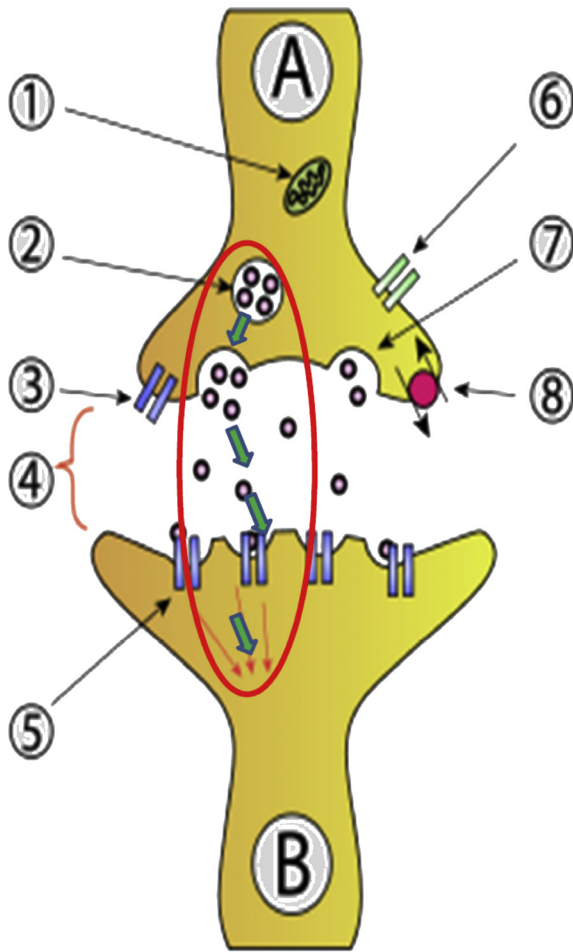
Fig. 1. Within mesolimbic neurons [A, B], trace nitrous oxide ( N_2O ) stimulates the release of opioid peptides, including dynorphin (DYN) A (1-17), contained within synaptic vesicles (2) and ultimately released into the synaptic membrane (4) via vesicular fusion (7). These peptides act on cognate opioid receptors such as the kappa opioid receptor (KOR) (6). Owing to aging, KOR constitutive expression declines, leaving the receptor more sensitive to chronic ligand-induced stimulation (i.e., downregulation). This receptor modulation permits DYN-induced activation of several nonopioid targets (indicated by multiple red arrows), including activation of \alpha -amino-3-hydroxy-5-methylisoxazole-4-propionate (AMPA)/kainate receptors (5), triggering an apoptotic pathway that involves cytochrome c release from mitochondrion (1), caspase-3 activation, and restricted calcium influx via inhibition of the \alpha 7 receptor (8), as well as leakage from phospholipid vesicles contained within the neuronal membrane in an attempt to restore free choline (See text). These AD-related effects are hypothesized to co-occur with the well-documented effects of N_2O on cobalamin and folate metabolism through the inactivation of the methionine synthase enzyme.
