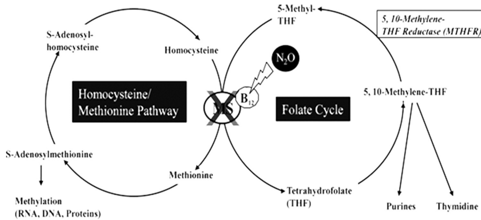
Fig. 2. A schematic showing N_2O -induced inactivation of methionine synthase in the folate-mediated one carbon metabolic pathway. (Figure from [57])
