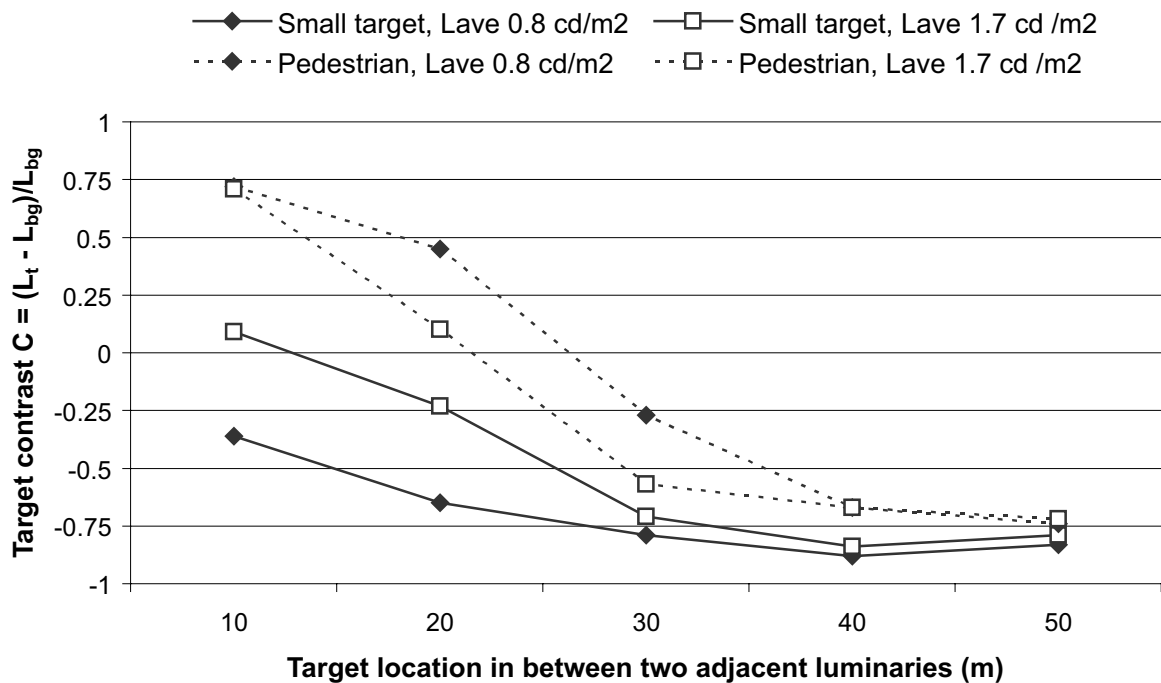
Figure 1 Contrasts of a small flat target ( 20 \text{ cm} \times 20 \text{ cm} , p = 0.2 ) and a pedestrian ( p = 0.16 ) when located at varying positions on the road and the roadside. The results represent two different road lighting conditions measured in dry weather conditions at Ring Road III Vantaa, Finland. The road surface was illuminated by 250 W high pressure sodium lamps with a pole spacing of 55 m. The target contrasts vary between C = -0.88 – 0.72 .
