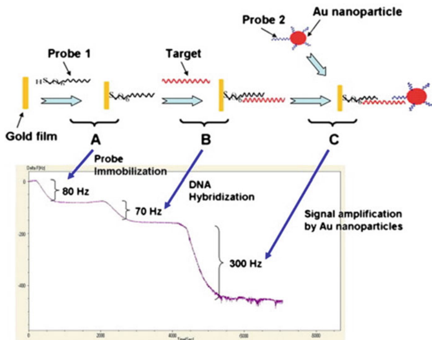
Fig. 7 Time-dependent frequency changes of the circulating-flow QCM sensor, (a) addition of Probe 1 (1 \mu\text{M} ; P1-30/12 T) for immobilization on the surface of the QCM sensor via self-assembly, (b) complementary target oligonucleotides [0.5 \mu\text{M} ; T-104(AS)] are subsequently introduced for DNA hybridization, (c) additional treatment of the DNA hybridized QCM with Probe 2 (P2-30/12 T)-capped Au nanoparticles. The sequences of Probe 1 and Probe 2 are complementary to the two ends of the analyte DNA (i.e., target sequences) (Reproduced from Chen et al. [72] with permission from Elsevier)
