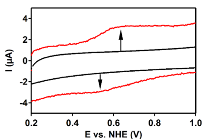
Figure 4. CV in a 100 mM pH 7 phosphate buffer at a scan rate of 100 mV/s before (black) and after (red) the electrode was cycled 75 times between 0.2 and 1.6 V versus NHE in a 0.5 mM Co(HL) in a 100 mM pH 7 phosphate buffer at a scan rate of 100 mV/s. GC, Au, and RHE were used as WE, CE, and RE, respectively. Potentials were converted to NHE.
