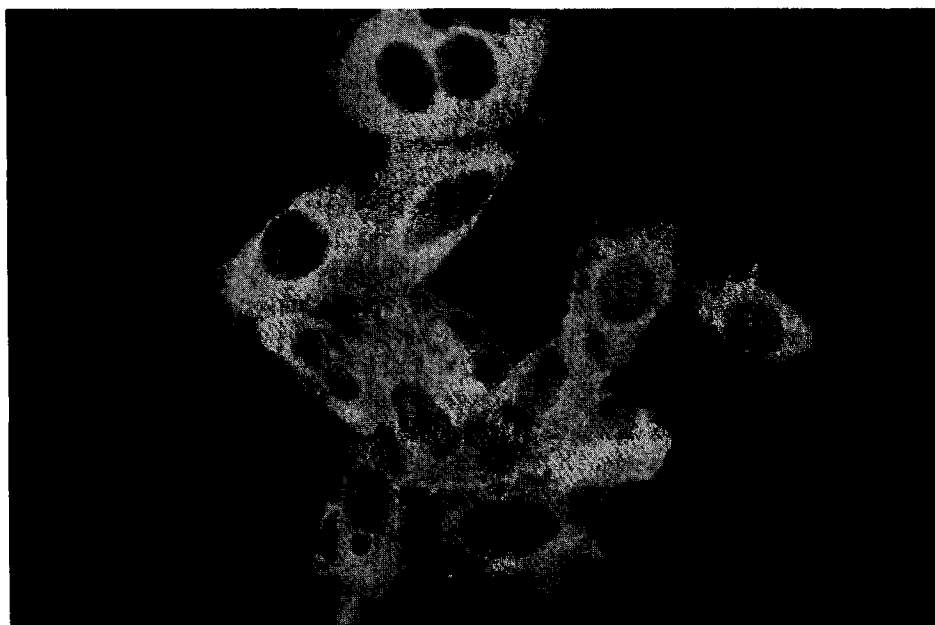
Fig. 3. Immunofluorescence staining of human coronavirus 229E-infected C16 cells using an infected volunteer serum.
