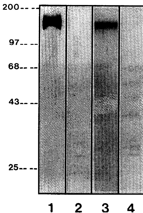
Fig. 2. Western blot analysis of purified carrier and fusion proteins using an infected volunteer serum. Lane 1, \beta -gal/HCV-N ( \beta -gal/human coronavirus-N); lane 2, \beta -gal 1-1023 ; lane 3, \beta -gal/HCV-S ( \beta -gal/human coronavirus-S); lane 4, \beta -gal 1-375 . The positions of molecular weight markers stained with India ink in a parallel strip are indicated.
