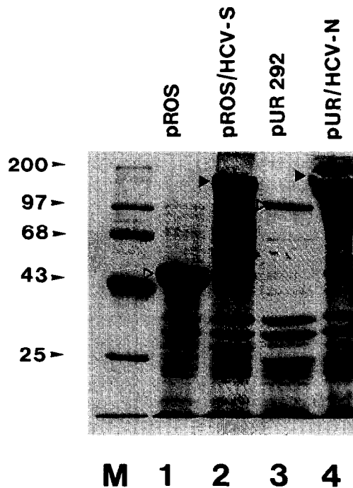
Fig. 1. SDS-PAGE analysis of bacterial expressed fusion proteins. Lane M, molecular weight marker; lane 1, pROS; lane 2, pROS/HCV-S (pROS/human coronavirus-S); lane 3, pUR 292; lane 4, pUR/HCV-N (pUR/human coronavirus-N). The position of the fusion proteins is indicated by a filled arrowhead. The position of the carrier protein is indicated by an open arrowhead.
