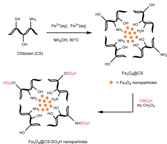
Scheme 1 Synthesis of \text{Fe}_3\text{O}_4@\text{CS-SO}_3\text{H} nanoparticles.
