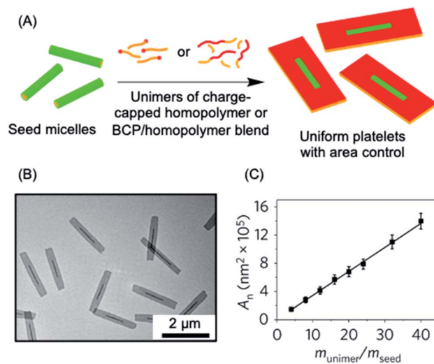
Fig. 3 2D living CDSA. (A) Schematic illustration of the living CDSA process in 2D to generate controlled area platelet micelles by the addition of a crystallizable charge-capped homopolymer or block copolymer (BCP)/homopolymer blends to 1D seed micelles. (B) Controlled area 2D platelet micelles from the addition of 20 mass equivalents of charge-capped PFDMS homopolymer to PFDMS- b -poly(2-vinylpyridine) seed micelles. (C) A plot showing the linear relationship between average platelet micelle area and unimer to seed mass ratio. Panels (B) and (C) reproduced from ref. 145.
