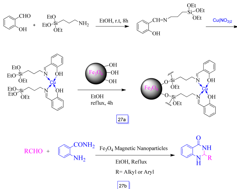
Scheme 27 Synthesis of \text{Fe}_3\text{O}_4 -Schiff base of \text{Cu}(\text{II}) (a) and synthesis of 2,3-dihydroquinazolin-4(1H)-ones in the presence of \text{Fe}_3\text{O}_4 magnetic nanoparticles and ethanol solvent at reflux conditions (b).
