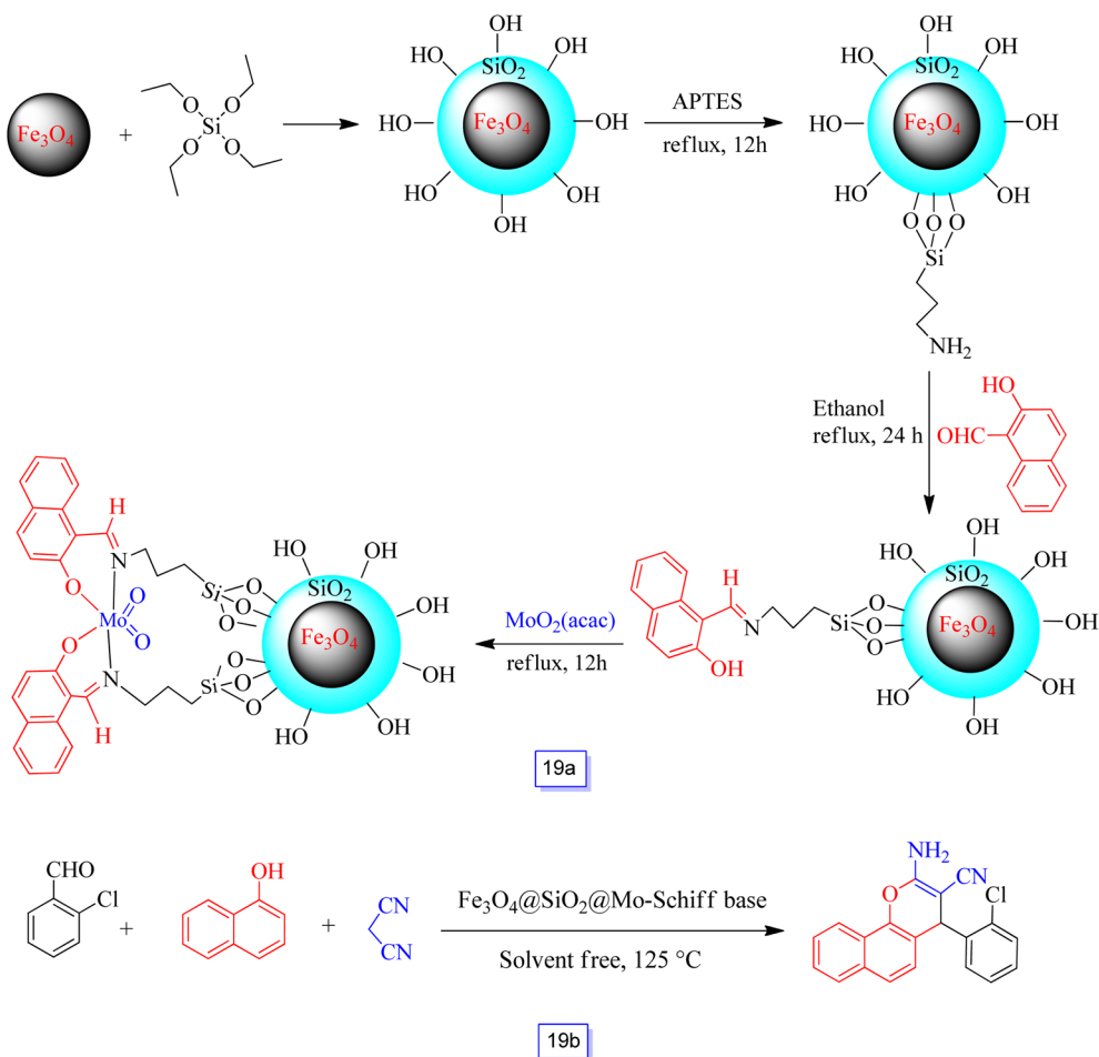
Scheme 19 Preparation of \text{Fe}_3\text{O}_4@\text{SiO}_2@\text{Mo-Schiff base} (a), and synthesis of 2-amino-4H-benzo[h]chromenes in the presence of \text{Fe}_3\text{O}_4@\text{SiO}_2@\text{Mo-Schiff base} at 125 °C under solvent free conditions (b).
