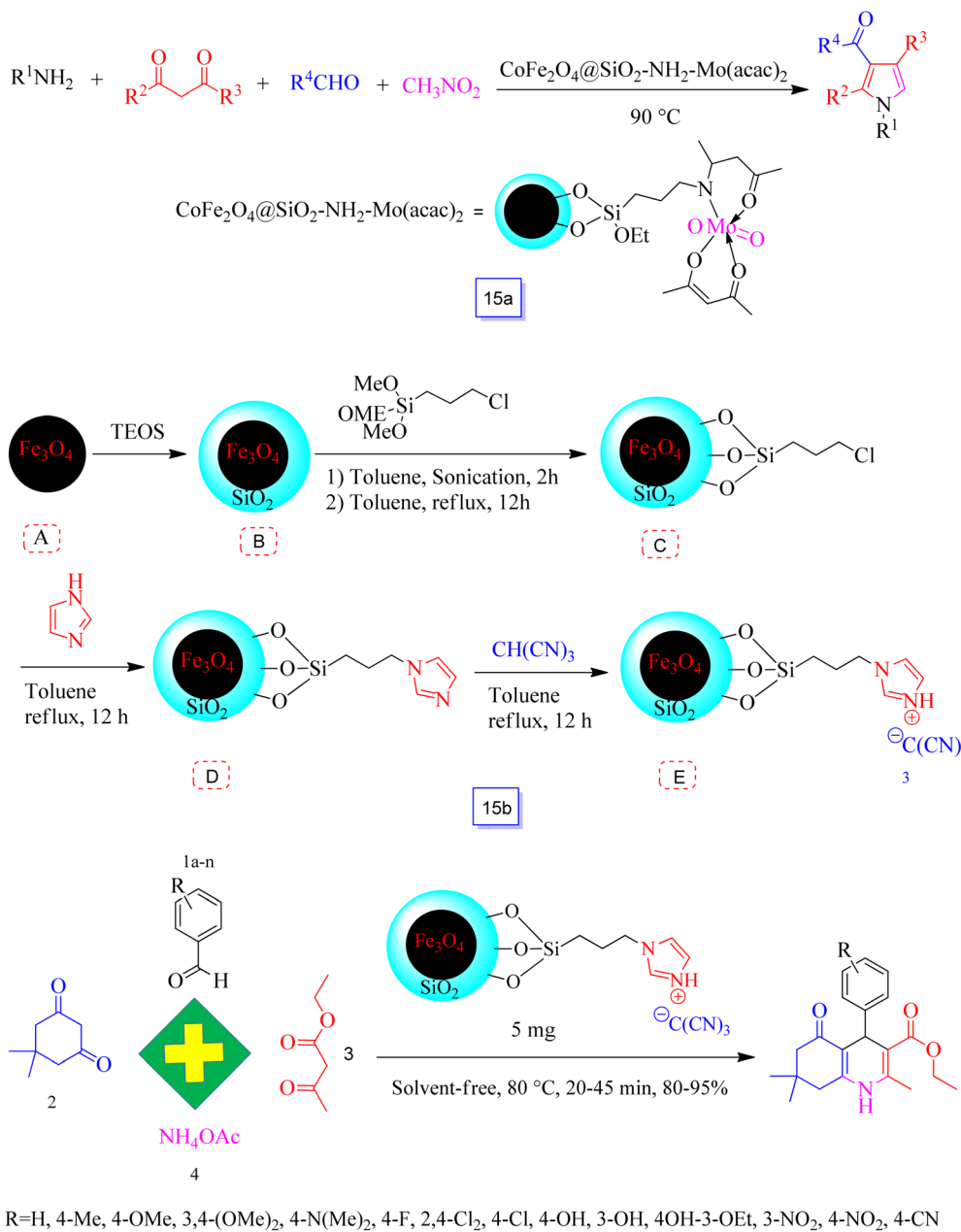
Scheme 15 Synthesis of functionalized pyrroles in the presence of CoFe_2O_4@SiO_2-NH_2-Mo(acac)_2 at 90 °C (a), preparation of \{Fe_3O_4@SiO_2@[(CH_2)_3Im]C(CN)_3\} (b), and synthesis of polyhydroquinoline derivatives in the presence of MNP_5@IL at 80 °C under solvent free conditions (c).
