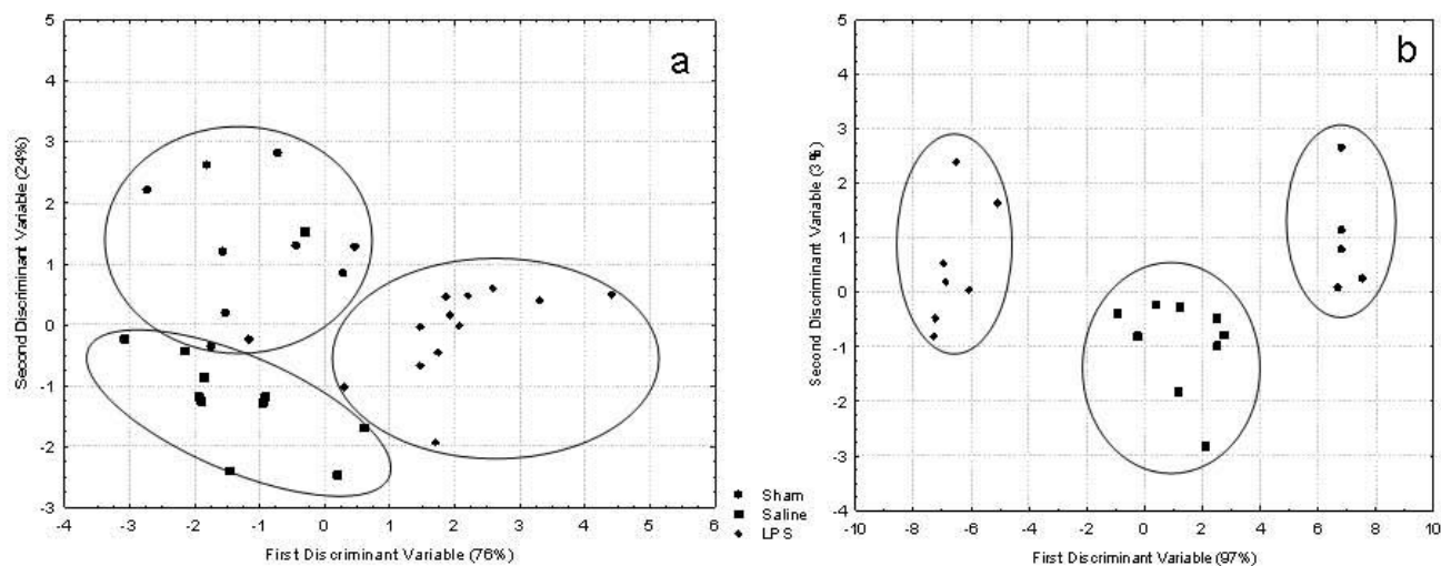
Figure 3 Immunostimulated bees display significantly different cuticular hydrocarbon chemical profiles. Discriminant analysis was performed on the cuticular chemical profiles of sham, saline- and lipopolysaccharide-injected honey bee workers based on their relative proportions of chemical compounds (a, colony SD18, F(14,46) = 5.69, P < 0.0001 ). Data were obtained from gas chromatography analysis of cuticular washes. Similar results were obtained for bees derived from a different colony in a second independent trial (b, colony SD11, ( F(26,10) = 6.74; P = 0.0016 ).
