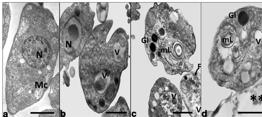
Fig. 6 Ultrastructural effects of the STLs on L. mexicana promastigotes. Parasites were incubated with medium alone (a) as negative control or 0.5 \mu g/ml of either enhydrin (b), polymatin B (c) or uvedalin (d). Magnification: 3200 \times (b-d); 3600 \times (a). Scale-bar: 1 \mu m. Abbreviations: N nucleus, Mc mitochondria, F flagellum, V vacuoles, Gl glycosomes, mL multilamellar structure; **, destroyed parasite
