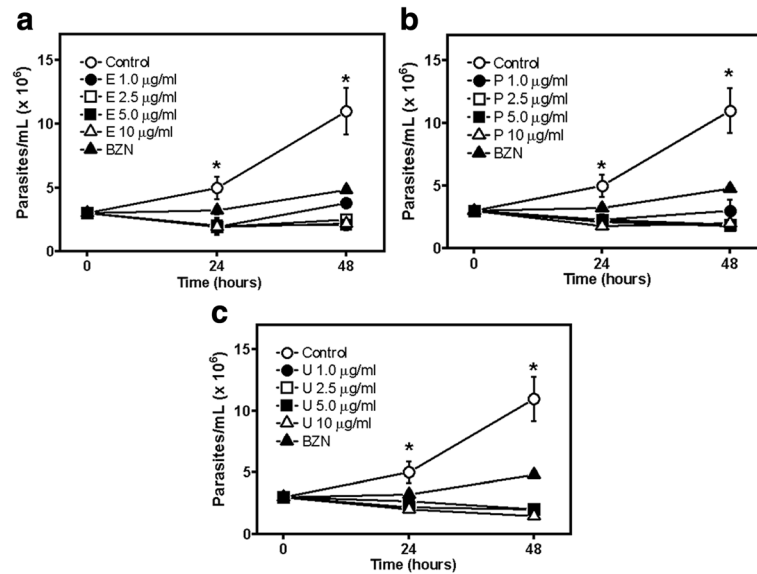
Fig. 3 Effect of enhydrin (a), polymatin B (b) and uvedalin (c) on the growth of T. cruzi epimastigotes (Dm28c) at the indicated concentrations, after 24 and 48 h of treatment. Symbols represent mean ± SEM from three independent experiments. BZN (5 μg/ml) was used as positive control and 1% DMSO was used as negative control. (*) above the means indicate significant differences ( P \leq 0.05 ) between control and compounds under study at 24 (a) and 48 h (b)
