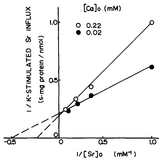
FIGURE 11. Effect of Sr concentration on ^{86}\text{Sr} influx with 0.02 (●) and 0.22 (○) mM Ca. Data are plotted in double reciprocal form. Measurements were at 1 s. The K_{m(\text{Sr})} value obtained by extrapolating the line joining the solid points to the intercept with the X axis was 2 mM (uncorrected). The K_{I(\text{Ca})} value obtained by extrapolation after correcting for competition with Sr was 0.22 mM.
