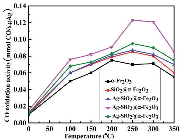
Fig. 10 Effect of CO oxidation activity in \alpha\text{-Fe}_2\text{O}_3 , \text{SiO}_2@\alpha\text{-Fe}_2\text{O}_3 , \text{Ag (1 wt\%)-SiO}_2@\alpha\text{-Fe}_2\text{O}_3 , \text{Ag (2 wt\%)-SiO}_2@\alpha\text{-Fe}_2\text{O}_3 and \text{Ag (3 wt\%)-SiO}_2@\alpha\text{-Fe}_2\text{O}_3 samples.
