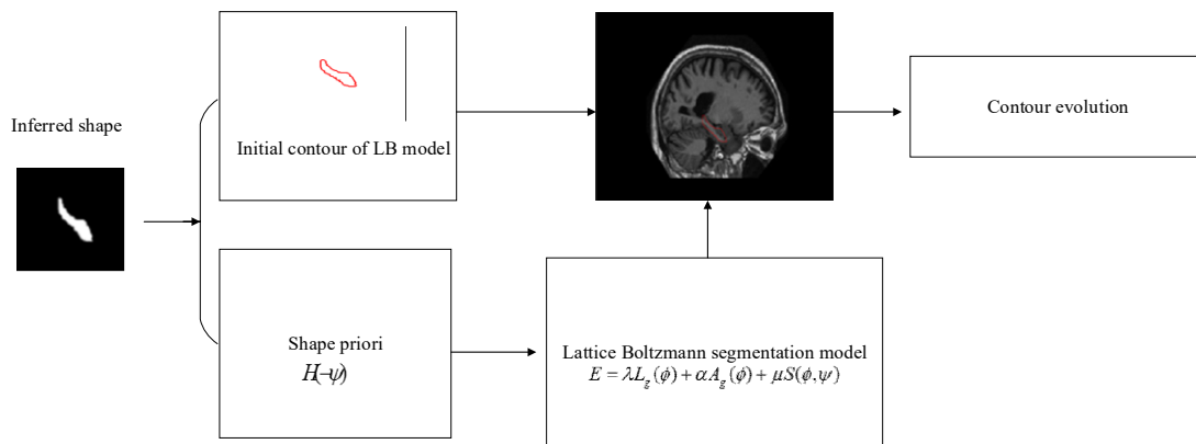
Figure 4. The flowchart of the LB segmentation model.
