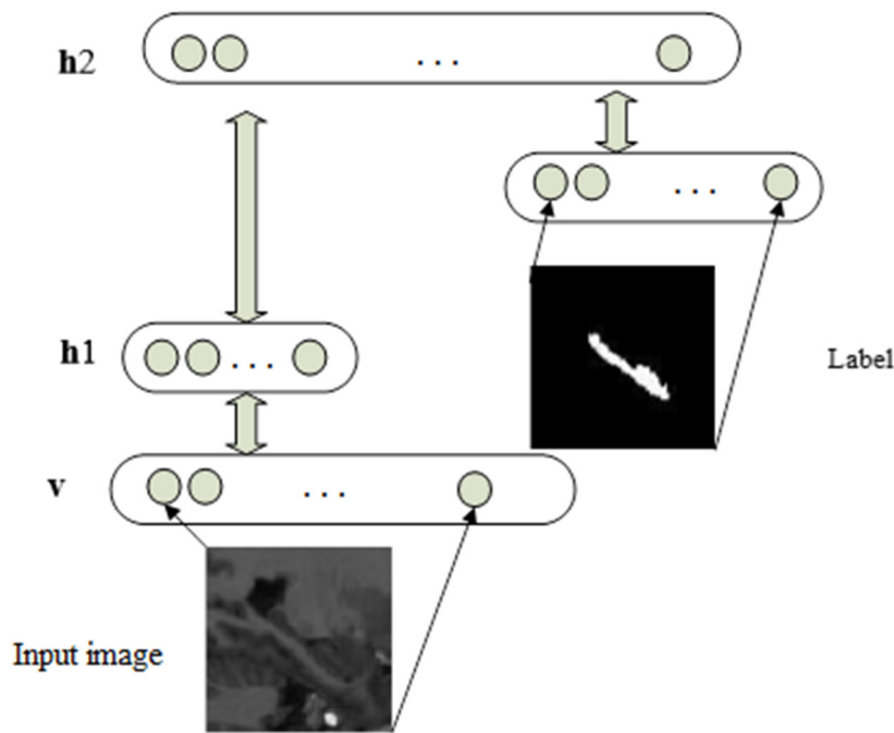
Figure 2. The deep belief network (DBN) used for shape inferring.
