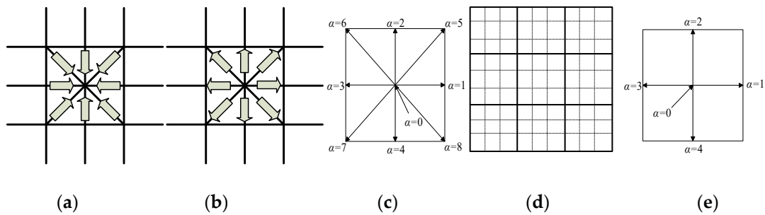
Figure 3. Explanation of the lattice Boltzmann (LB) method for image processing. (a) Collision process; (b) streaming process; (c) D2Q9 structure; (d) sub-pixel denoted by dotted box and pixel denoted by solid box; (e) D2Q5 structure.
