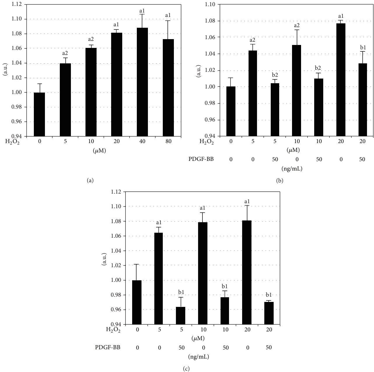
FIGURE 2: Effects of PDGF-BB on H 2 O 2 -induced calpain activation. Calpain-1 activity was measured 24 h after exposure to H 2 O 2 as described in the Experimental procedures. (a) Calpain activity induced by the indicated amounts of H 2 O 2 (5, 10, 20, 40, and 80 μM) exposure increased calpain activation in cortical neurons in a dose-dependent manner from 5–20 μM. ((b), (c)) Calpain activity in neuronal cultures pretreated with 50 ng/mL PDGF-BB 24 h (b) and 48 h (c) before exposure to H 2 O 2 PDGF-BB completely blocked calpain activity induced by H 2 O 2 . Data are expressed as means ± SEM of three independent experiments. a1 P < 0.01 and a2 P < 0.05 versus the untreated control; b1 P < 0.01 and b2 P < 0.05 versus the same H 2 O 2 exposure without the PDGF-BB pretreatment.
