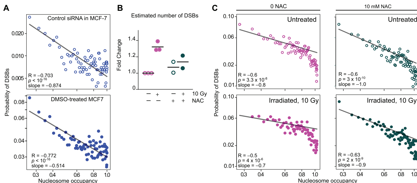
Figure 5. DSBs anti-correlates with nucleosome occupancy in human MCF-7 cells. (A) Interrogation of public datasets: The probability of harboring endogenous DSBs anticorrelates with nucleosome occupancy. This hypothesis was tested on BLISS and ATAC datasets produced and published by other groups: ATAC-seq GSE101736, GSM2714245; BLISS GSE136365, GSM4047452 (left) and GSM4047456 (right). Each dot represents one percentile in nucleosome occupancy. The x -axis, log scale, is the nucleosome occupancy value; the y -axis, log scale, is the probability to harbor one or more DSBs. Statistics: Pearson correlation on the log-transformed values. (B) Estimated number of DSBs in MCF-7 cells, expressed as fold change over the paired control sample (not treated not irradiated). MCF-7 cells were pre-treated (magenta) or not (green) with 10 mM N -acetyl-L-cysteine (NAC) for 1 h and irradiated or not with 10 Gy; dots and lines represent biological replicates and averages, respectively. Statistics: two-way ANOVA test (paired experiments). Irradiation dose ( P = 0.0063 ) and interaction of irradiation and NAC treatment ( P = 0.043 ) are statistically significant; NAC treatment ( P = 0.28 ) is not. (C) The probability of harboring DSBs anticorrelates with nucleosome occupancy. Each dot represents one percentile in nucleosome occupancy (ATAC-seq raw data from GSE101736). The x -axis, log scale, is the nucleosome occupancy value; the y -axis, log scale, is the probability to harbor one or more DSBs. Statistics: Pearson correlation on the log-transformed values.
