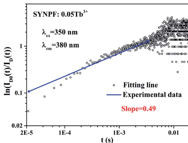
Fig. 8 The relationship of \ln(I_{D_0}(t)/I_D(t)) vs. t plotted in a double logarithmic coordinate for sample SYNPF:0.05 Tb^{3+} .
