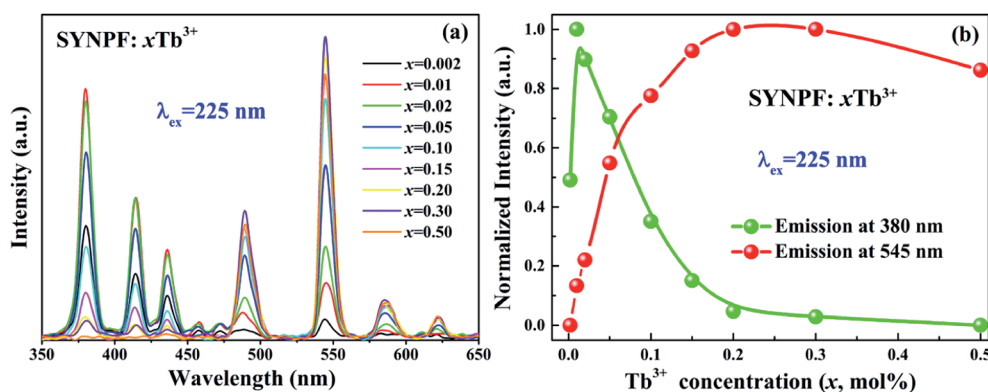
Fig. 3 Dependence of the (a) PL ( \lambda_{ex} = 225 nm) spectra and (b) emission intensity of Tb 3+ in SYNPF phosphors with the variation of Tb 3+ concentrations.
