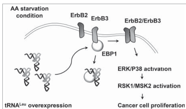
Figure 7. Schematic representation for the role of free tRNA Leu . Under amino acid starvation condition, free tRNA Leu interacts with EBP1 and enhances the activation of ErbB2/ErbB3 pathway. Finally, the downstream signaling mediated by RSK1/MSK2 facilitates cancer cell proliferation.
