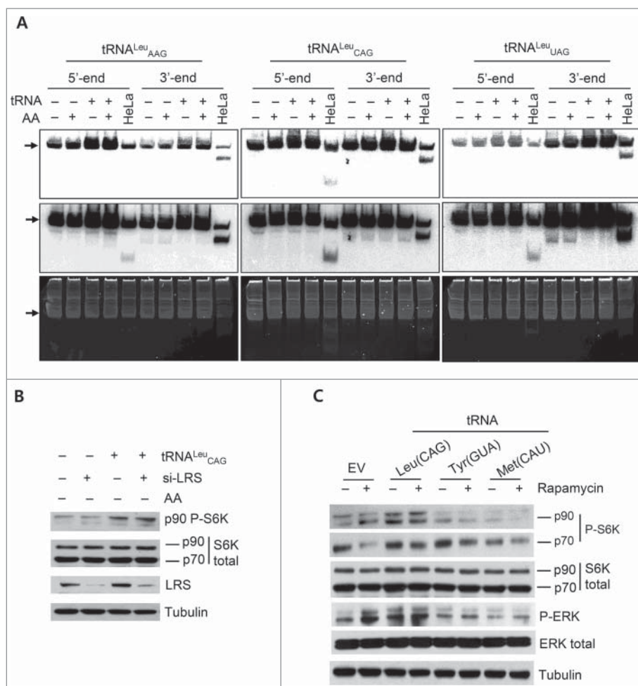
Figure 3. Phosphorylation of 90-kDa RPS6K was mediated by mature tRNA Leu , and it was independent of mTOR activation. (A) Northern blot analysis to detect both mature tRNA Leu and its tRFs with 5' and 3' radioactive short probes. Expression levels of tRNAs in HEK 293T cells after tRNA Leu transfection under different culture conditions were compared with that in the controls. Arrows show the mature tRNA. Upper, short exposure; middle, long exposure; and bottom, EtBr staining of the gel to visualize the loading amounts of total RNA. HeLa cells were used as controls for tRFs. (B and C) Western blot analysis to investigate the effect of LRS knockdown (B) or rapamycin treatment (C) on the tRNA-mediated p90 RPS6K phosphorylation.
