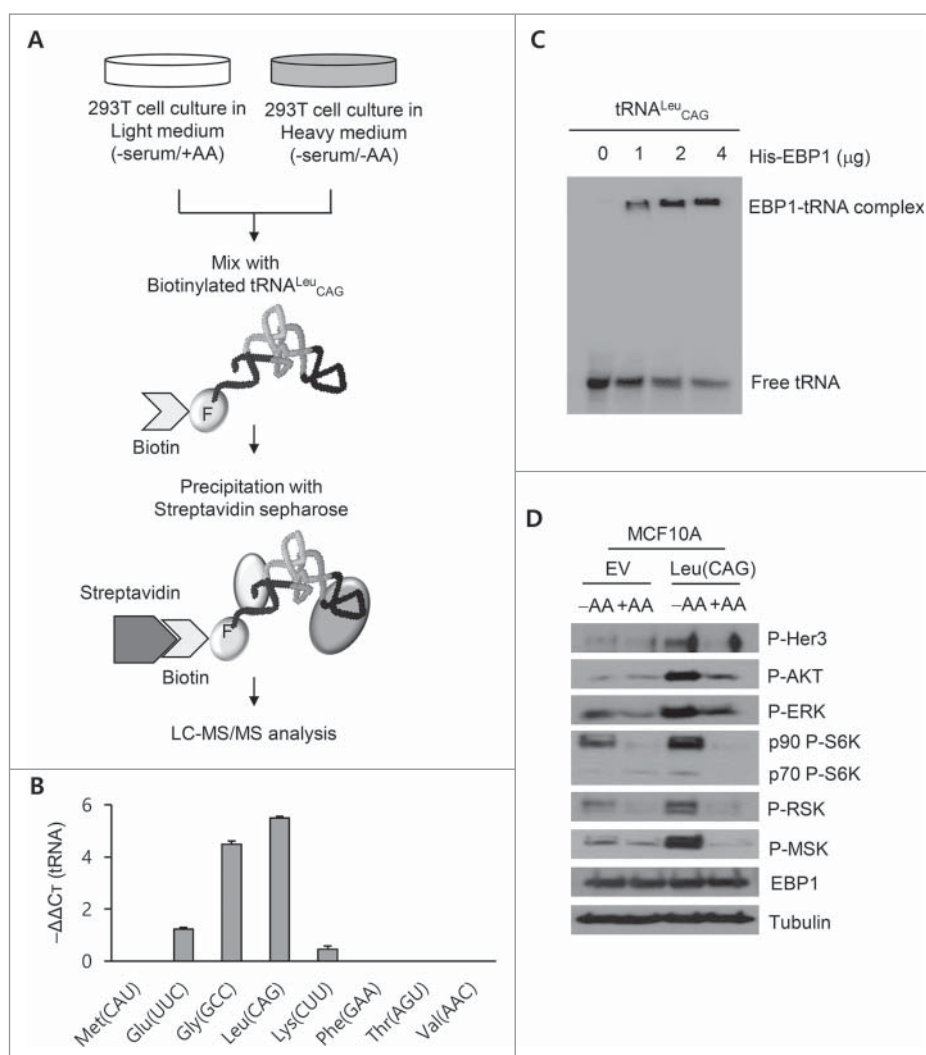
Figure 5. Interaction between EBP1 (ErbB3-binding protein 1) and tRNA Leu . (A) Schematic diagram for the process of SILAC and LC-MS/MS analysis. Synthesized tRNA Leu CAG was biotinylated by incubation with biotin-Phe-DME and flexizyme. After isolating the tRNA Leu CAG -associated protein complexes via biotin-streptavidin interaction, the proteins were analyzed by LC-MS/MS. F, Phenylalanine. (B) qRT-PCR analysis to detect the tRNAs associated with immunoprecipitated EBP1 from the HEK 293T cells incubated in amino acid-free media. Values are presented as means ± standard deviations (n = 3). (C) Gel shift assay to detect the formation of the complex between EBP1 and radioactively synthesized tRNA Leu CAG . (D) Western blot analysis for the ErbB3 signaling pathway of MCF10A cell lines transfected with tRNA Leu . -AA, amino acid starvation; +AA, amino acid supplementation.
