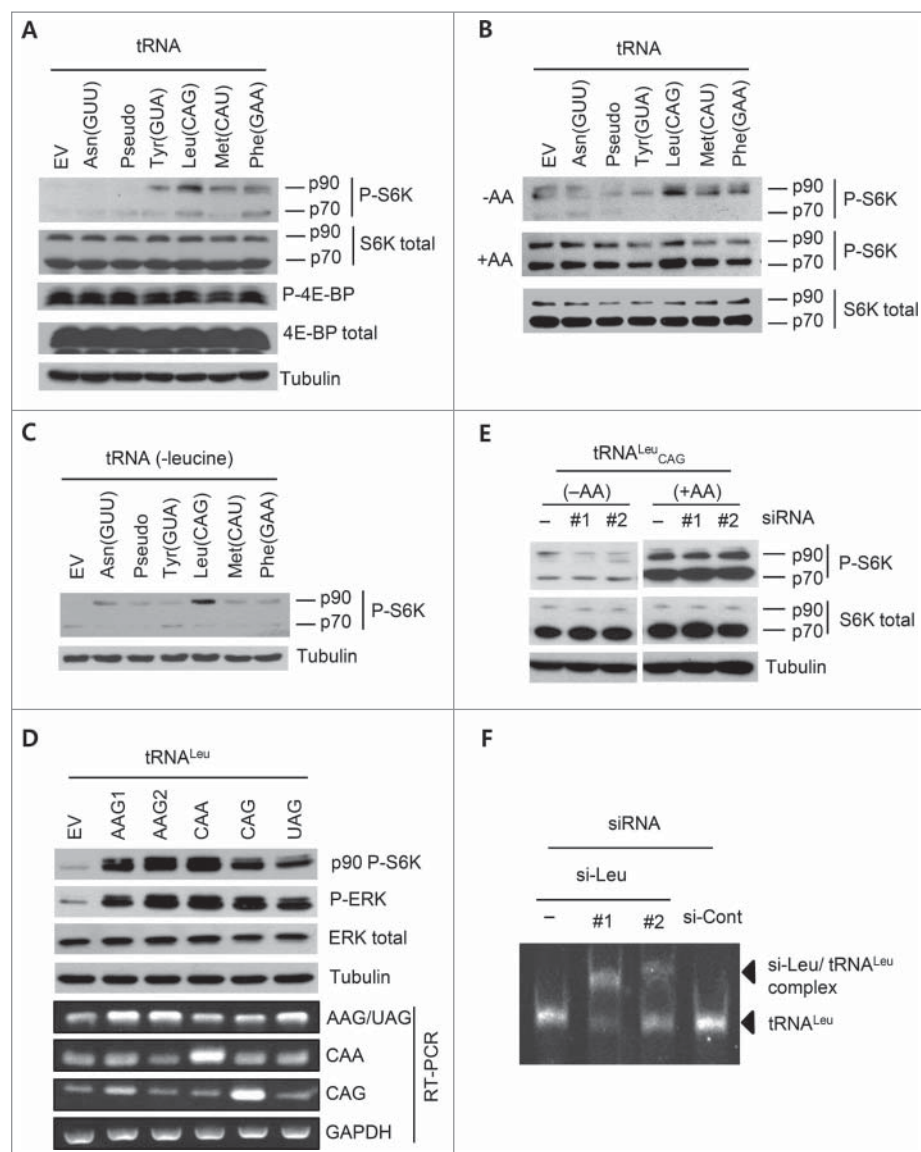
Figure 2. Overexpression of tRNA Leu induced the phosphorylation of 90-kDa RPS6K under amino acid starvation. (A and B) Western blot analysis of HEK 293T cells transfected with different tRNAs. Phosphorylation of S6K and 4E-BP, P-S6K and P-4E-BP, respectively, were analyzed without media change (A) and after incubation under amino acid-deprivation for 3 h as well as after addback of amino acids and further incubation for 1.5 h (B). Phosphorylation signals in the 90-kDa (p90) and 70-kDa (p70) sizes detected by p70 S6K specific antibody (P-S6K) are shown. tRNA-like pseudo RNA was also included. -AA, amino acid starvation; +AA, amino acid supplementation. Tubulin, total S6K, or total 4E-BP were used as controls. (C) P-S6K was analyzed via western blot with HEK 293T cell lysates transfected with tRNA for 24 h, and then incubated with leucine-free media for 3 h. (D) Western blot and RT-PCR analyses for the cell lysates transfected with tRNA Leu isotypes. Two tRNA Leu AAG vectors with different flanking sequences, but the same tRNA gene, were included. P-S6K and ERK phosphorylation (P-ERK) were detected after overexpression of each tRNA. Tubulin and GAPDH were used as controls. (E) Western blot analysis for the tRNA Leu CAG -overexpressing cell lysates transfected with tRNA Leu CAG -specific siRNA (si-Leu). Two different si-Leu sequences were used here. -AA, amino acid starvation; +AA, amino acid supplementation. (F) Gel shift assay to monitor the formation of the complex between tRNA Leu CAG and si-Leu. si-Cont, si-Control.
