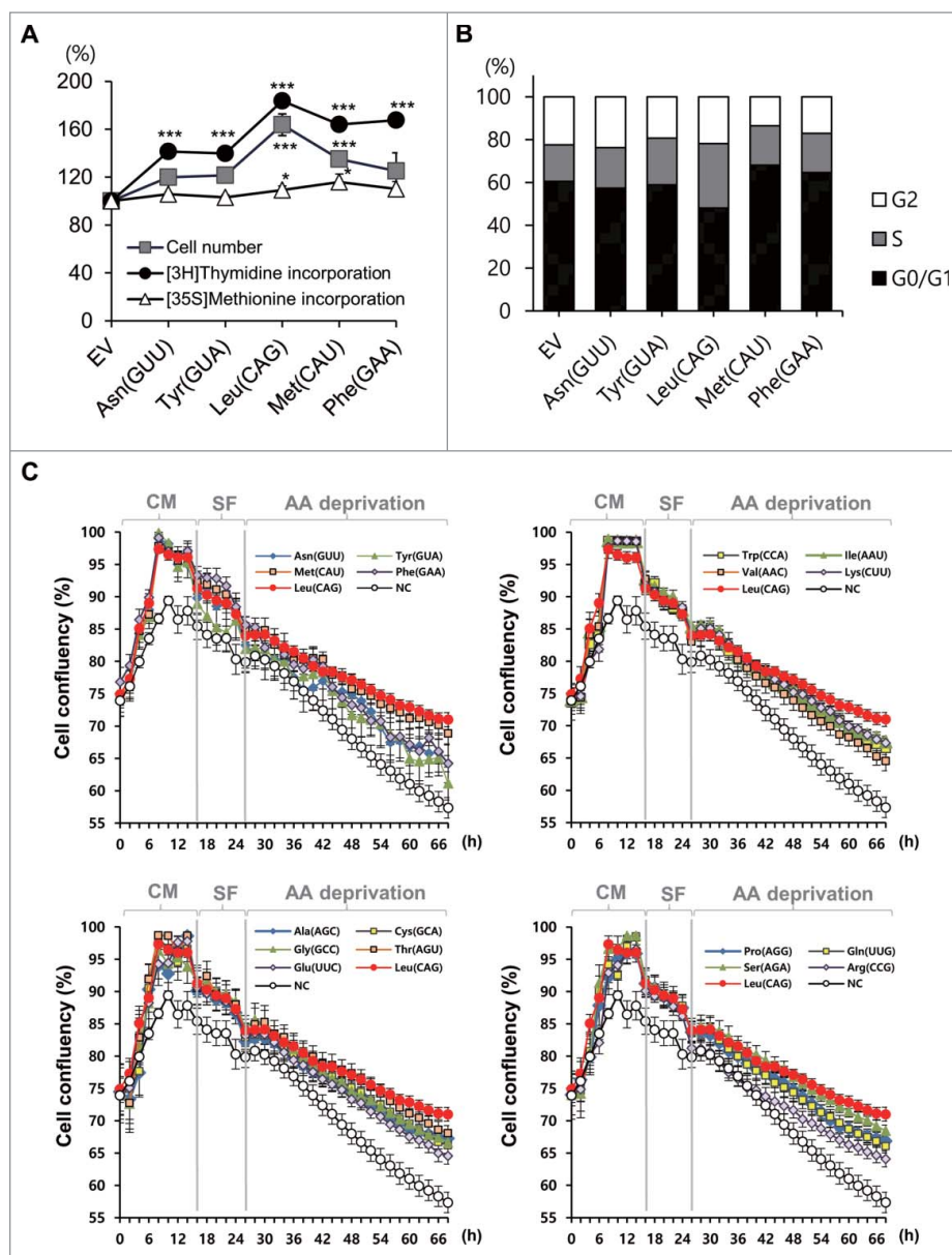
Figure 1. Overexpression of tRNAs enhanced the cell proliferation. (A) Relative levels (percentage) of cell number, thymidine incorporation, and methionine incorporation after overexpression of each tRNA were compared with those in EV (empty vector)-transfected control. Values are presented as means \pm standard deviations ( n = 3 ). *, P < 0.05 ; ***, P < 0.001 . (B) Change in cell cycle after tRNA transfection was compared with that in control. (C) Real-time proliferation of HEK 293T cells transfected with different tRNAs was monitored under different culture conditions. Values are presented as means \pm standard errors ( n = 9 ). Values for tRNA Leu CAG and negative control (NC) are repeated in all the graphs for the comparison. Cell viability was calculated as the relative percentage of confluency. CM, complete media; SF, serum free; AA, amino acids.
