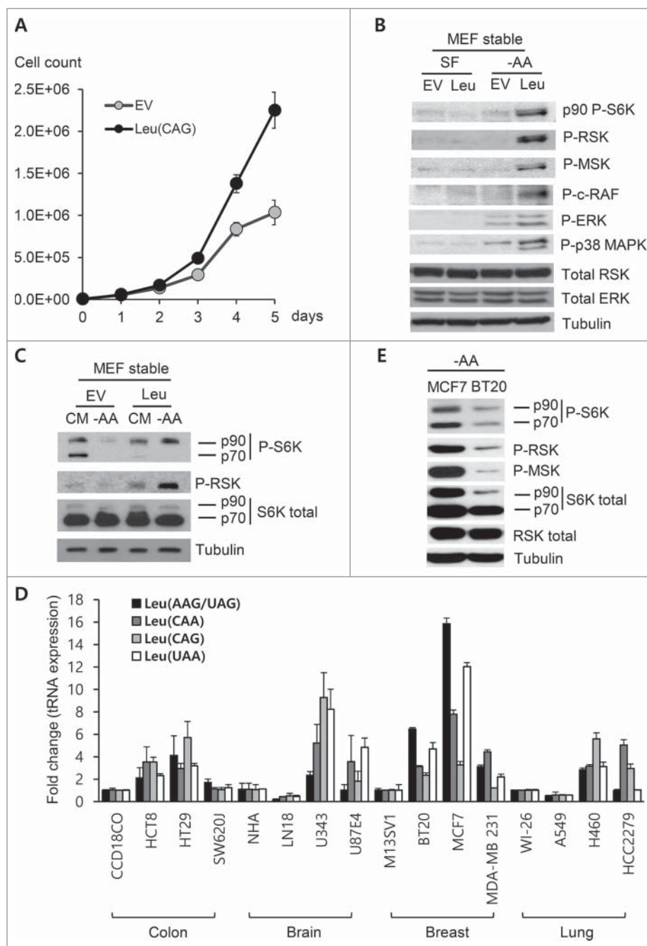
Figure 6. Characteristics of stable tRNA^{Leu}_{CAG} -overexpressing cells. (A) Real-time monitoring of the proliferation of stable NIH3T3 MEF cells expressing tRNA^{Leu}_{CAG} . Values are presented as means \pm standard deviations ( n = 9 ). (B and C) Western blot analysis of the stable NIH3T3 MEF cells under different culture conditions. Activation of RSK and MSK signaling was compared under SF (serum free) and -AA (amino acid starvation) (B) or under CM (complete media) and -AA (amino acid starvation) conditions (C). (D) Levels of the different tRNA^{Leu} isotypes in several cancer cell lines were analyzed using qRT-PCR and then compared with those in normal cell lines (CCD18CO, NHA, M13SV1, and WI-26). Values are presented as means \pm standard deviations ( n = 3 ). (E) Comparison of RSK and MSK signaling between MCF7 and BT20 cell lines under amino acid-deprived conditions ( -AA ).
