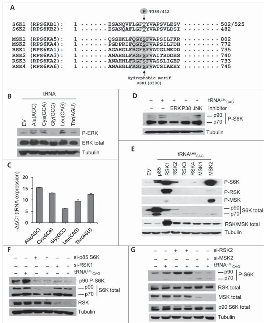
Figure 4. RSK1 and MSK2 were the 90-kDa RPS6K phosphorylated by tRNA Leu CAG overexpression. (A) Sequence alignment of 8 different RPS6 family kinases. The hydrophobic motif and representative phosphorylation sites are shown in gray and indicated by arrows, respectively. The 502 aa and 525 aa sizes in S6K1 indicate p70 S6K and p85 S6K, respectively. (B and C) Effect of tRNA overexpression on the ERK phosphorylation (B) and qRT-PCR analysis to detect tRNA overexpression (C). Values are presented as means \pm standard deviations ( n = 3 ). (D) The effect of ERK (U0126), p38 MAPK (SB203580), and JNK (SP600125) inhibitors on the tRNA Leu CAG -mediated p90 RPS6K phosphorylation. (E-G) Western blot analysis for the phosphorylation of RPS6K after overexpression of tRNA Leu and the different RPS6 family kinases (E), after siRNA transfection specific to p85 S6K and RSK1 (F) as well as RSK2 and MSK2 (G).
