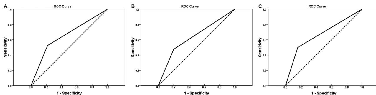
Figure 3 EAAT1, DHFR, and fetuin-A ROC curves for overall survival in CS patients (N = 80) from January 2011 to June 2015. AUCs for EAAT1 (A), DHFR (B), and fetuin-A (C) were 0.654, 0.638, and 0.670, respectively, indicating good predictive performance.
