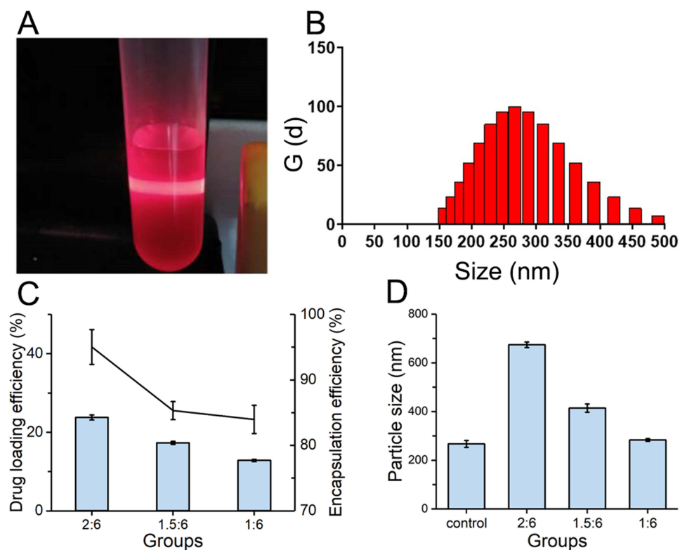
Figure 2 The preparation and characterization of Fc^+-C_{18}@CUR : (A) Tyndall effect and (B) particle size of blank Fc^+-C_{18} micelle particles. (C) Drug loading efficiency and encapsulation efficiency and (D) particle size of three formulations with different mass ratio between CUR and Fc^+-C_{18} .
