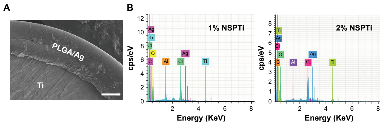
Figure 2 EDS scanning along the cross-section of nanosilver/PLGA coating (A). Elements in nanosilver/PLGA coatings detected by EDS (B). White scale bar =20 \mu\text{m} . Abbreviations: EDS, energy-dispersive spectroscopy; NSPTi, nanosilver/poly (DL-lactic-co-glycolic acid)-coated titanium; PLGA, poly (DL-lactic-co-glycolic acid).
