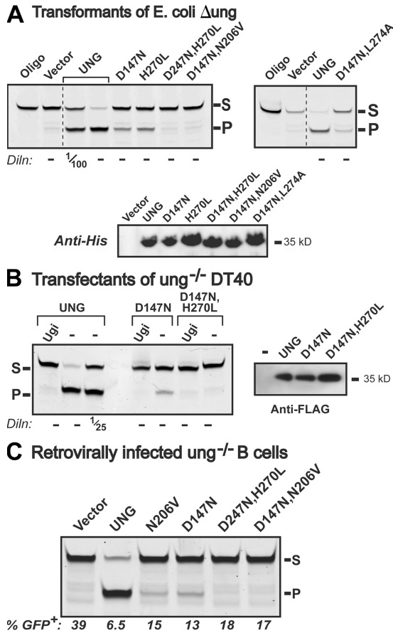
Figure 3. Mutant UNGs that support switching retain uracil-excision activity. (A) Assay for uracil-excision activity by recombinant UNGs produced in E. coli . 10 \mu g extracts of E. coli ( \Delta ung) transformants expressing His-tagged versions of the indicated mouse UNG variants were incubated with 0.5 pmol of FITC-labeled, U-containing single-stranded oligonucleotide substrate. After incubation with apyrimidinic endonuclease and subsequent PAGE, uracil excision is evident from conversion of the fluorescently labeled 42-mer substrate (S) into the 26-mer product (P). Undiluted extracts were used, except where indicated. A Western blot using an anti-histidine tag antiserum was used to control for expression levels. (B) Assay for uracil-excision activity in extracts of ung -/- DT40 cells transfectants expressing wild-type or mutant FLAG-tagged mouse UNGs. Samples (5 \mu g protein, or a dilution where specified) of whole-cell extracts were assayed for uracil-excision activity as described in A, but with the extracts preincubated with the UNG-specific inhibitor Ugi where indicated. (right) An anti-FLAG Western blot to control for expression levels. (C) Assay for uracil-excision activity in extracts of ung -/- mouse B cells that have been transduced with the indicated UNG-expressing retroviral vectors. Extracts (which were assayed undiluted) were prepared 4 d after retroviral transduction, and the proportion of retrovirally infected cells (as judged by GFP fluorescence) in each population is indicated below each lane. Endogenous SMUG1 activity was neutralized by preincubating the extracts with anti-SMUG1 PSM1 antibody (11).
