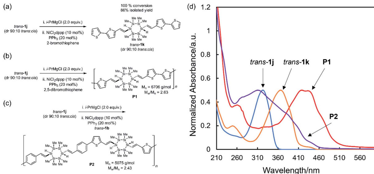
Fig. 7 (a) Model reaction: Kumada cross-coupling of trans\text{-}1j and 2-bromothiophene. (b) Kumada polycondensation synthesis of P1 . (c) Kumada polycondensation synthesis of P2 . (d) Comparison of UV-vis spectra of trans\text{-}1j (blue), trans\text{-}1k (orange), P1 (red) and P2 (purple) in THF. [ trans\text{-}1j ] = 10^{-5} M, [ trans\text{-}1k ] = 10^{-5} M, [ P1 ] = 0.03 g L ^{-1} , [ P2 ] = 0.03 g L ^{-1} .
