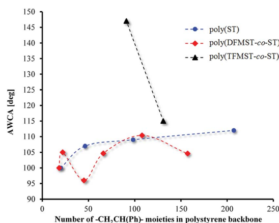
Fig. 6 Advancing water contact angles as function of the number of styrene moieties in polymers and copolymers.
