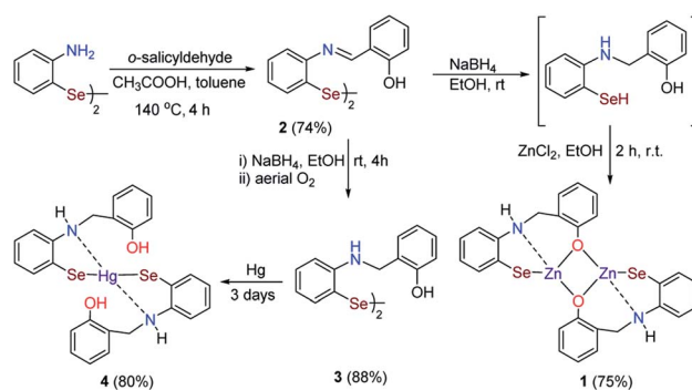
Scheme 2 Synthesis of zinc and mercuric selenolate 1 and 4 .
