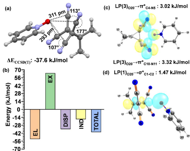
Fig. 3 (a) Fully optimized structure of the PNO:DMTCCP complex at the RI-B97D3/def2-TZVPP level of theory. The binding energy at the CCSD(T) level is -37.6 kJ mol ^{-1} . (b) The energy decomposition analysis shows that the interaction is dominated by electrostatic and dispersion. (c) Natural bond orbital (NBO) overlaps between the lone pairs of electrons of PNO–oxygen and the \pi^* -orbital of the nitrile bond of DMTCCP: n \rightarrow \pi^* interaction. (d) NBO overlap between the lone pairs of electrons of PNO–oxygen and the \sigma^* -orbital of the C _1 –C _2 bond of DMTCCP: n \rightarrow \sigma^* interaction.
