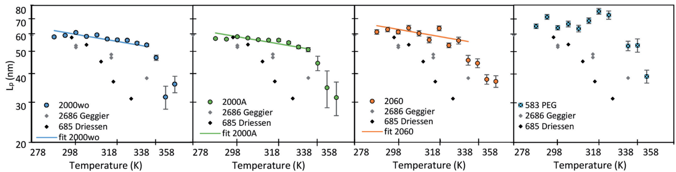
Figure 4. Temperature dependence of L_p for DNA molecule of 2000 bp without A_{50} tract (●) and 2000 bp with A_{50} (●), 2060 bp (●), and 583 bp on a PEG surface (x), as well as the results obtained by Geggier et al. on a 2686 bp circular DNA, as well as those obtained by Driessen et al. on a 685 bp linear DNA. Fits performed between 15 and 60°C by L_p = \kappa/k_B T with k_B = 1.38 \times 10^{-23} \text{ JK}^{-1} and \kappa as a fitting parameter, are shown when possible. Data are represented with logarithmic scales for both axes. Error bars (95% confidence intervals) are displayed, if not, they are smaller than the symbol size.
