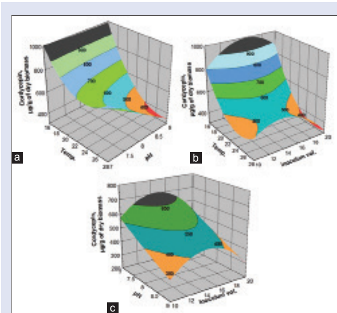
Figure 5: Response surface plots showing the (a) Effect of temperature and pH; (b) effect of temperature and inoculum volume; (c) pH and inoculum volume on cordycepin yield
