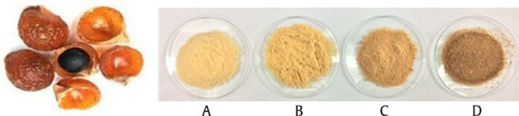
Fig. 1. Sapindus mukorossi fruits and dried extracts from ethanol (A), methanol (B), butanol (C) and distilled water (D).
