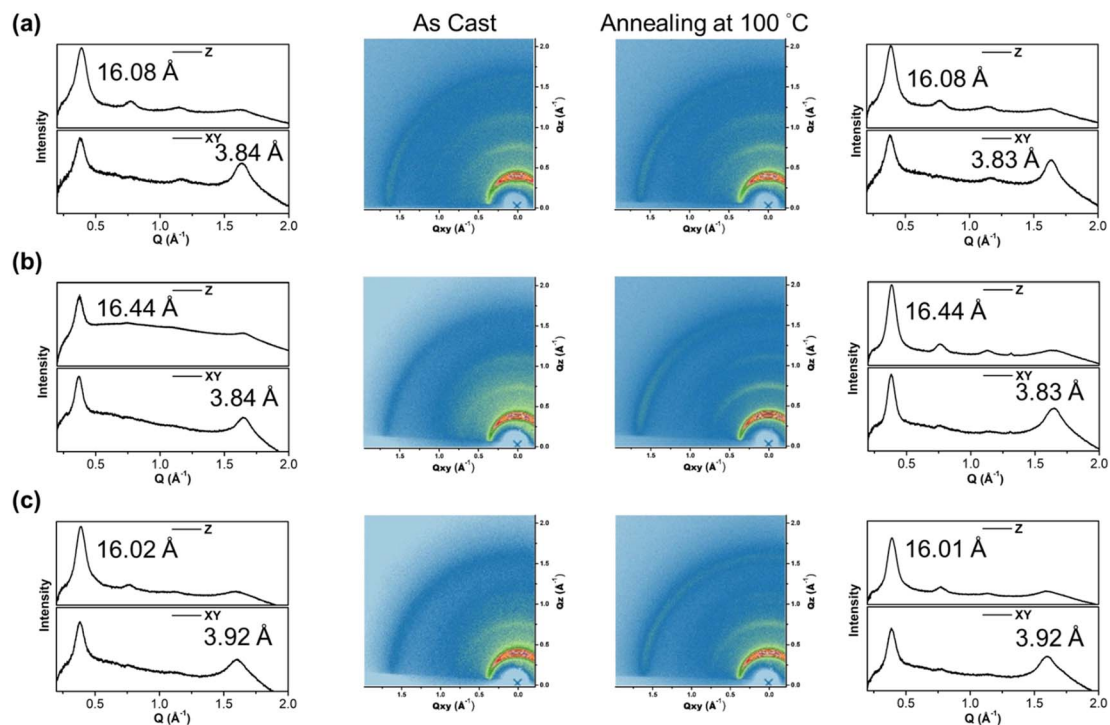
Fig. 6 (a) P(SSe) b (STe), (b) P(SSe) b (SeTe), and (c) P(STe) b (SeTe) 2D-GIWAXS images of the polymer thin films measured before and after thermal annealing at 100 °C and their corresponding 1D in-plane (bottom) and out-of-plane (up) linecuts.
