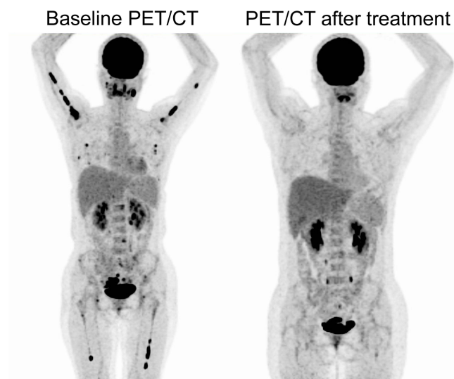
Figure 2 ^{18}\text{F} -FDG PET/CT imaging after and before treatment.
