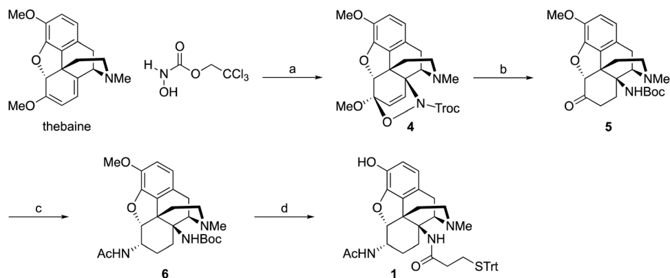
Scheme 1 Synthesis of hapten 1 . Reagent and conditions: (a) \text{NaIO}_4 , aq. \text{NaOAc}/\text{EtOAc} , 23\text{ }^\circ\text{C} , 96%. (b) (i) \text{Pd}/\text{C} , \text{H}_2 , \text{AcOH}/\text{NaOAc}/\text{MeOH} , 23\text{ }^\circ\text{C} . (ii) \text{Boc}_2\text{O} , \text{NaHCO}_3 , \text{THF}/\text{H}_2\text{O} , 0 to 23\text{ }^\circ\text{C} , 53%. (c) (i) \text{NH}_3 , \text{Ti}(\text{O}-i\text{Pr})_4 , \text{CH}_2\text{Cl}_2 , 0 to 23\text{ }^\circ\text{C} . (ii) \text{NaBH}_4 , \text{CH}_2\text{Cl}_2 , 23\text{ }^\circ\text{C} . (iii) \text{Ac}_2\text{O} , \text{Et}_3\text{N} , \text{CH}_2\text{Cl}_2 , 23\text{ }^\circ\text{C} , 81%. (d) (i) \text{BBr}_3 , \text{CH}_2\text{Cl}_2 , -78 to 23\text{ }^\circ\text{C} . (ii) 3-(tritylthio)propanoic acid, TBTU, \text{Et}_3\text{N} , 0 to 23\text{ }^\circ\text{C} , 29%.
