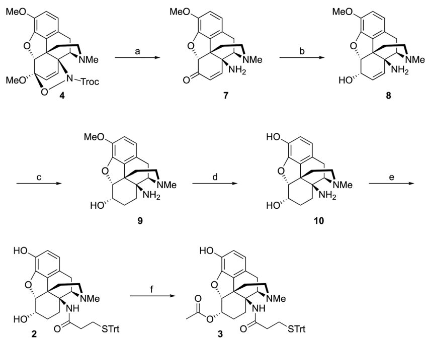
Scheme 2 Synthesis of 2 and 3 . Reagent and conditions: (a) (i) CSA, ethylene glycol, 23\text{ }^\circ\text{C} . (ii) \text{Zn} , (\text{NH}_4)_2\text{CO} , 100\text{ }^\circ\text{C} . (iii) \text{HCl} , \text{MeOH}/\text{H}_2\text{O} , 80\text{ }^\circ\text{C} , 47%. (b) \text{NaBH}_4 , \text{MeOH} , 23\text{ }^\circ\text{C} , quant. (c) \text{Pd}/\text{C} , \text{H}_2 , \text{MeOH} , 23\text{ }^\circ\text{C} , 81%. (d) \text{BBr}_3 , \text{CH}_2\text{Cl}_2 , -78\text{ }^\circ\text{C} , 84%. (e) 3-(tritylthio)propanoic acid, TBTU, \text{Et}_3\text{N} , \text{DMF} , 0\text{ }^\circ\text{C} . (ii) \text{KOH} , \text{EtOH}/\text{THF} , 80\text{ }^\circ\text{C} , 45%. (f) \text{Ac}_2\text{O} , DMAP, \text{Et}_3\text{N} , \text{CH}_2\text{Cl}_2 , 0\text{ }^\circ\text{C} , 39%.
