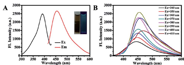
Fig. 1 (A) The fluorescence excitation and emission spectrum of AA-Cu NCs; (B) The fluorescence emission spectra of AA-Cu NCs under different excitation wavelength.
