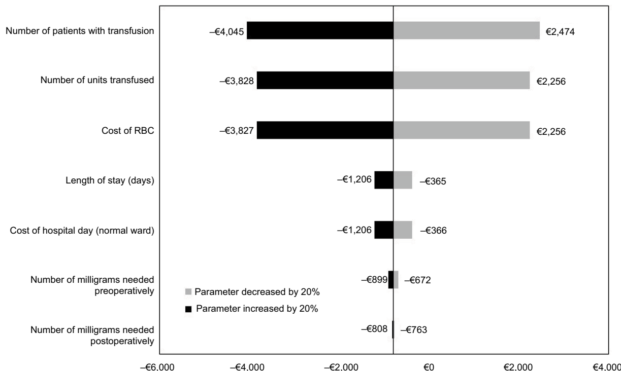
Figure 1 One-way sensitivity analysis results on the cost difference of FCM vs usual care based on individual case. Abbreviations: FCM, ferric carboxymaltose; RBC, red blood cell.
