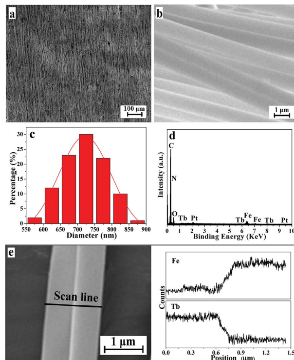
Fig. 2 SEM images at low magnification (a) and high magnification (b) of the JNAP. Diameter distribution histogram of the nanofibers in the JNAP (c). EDS spectrum of the JNAP (d). EDS line-scan analysis of a single Janus nanofiber in the JNAP (e).
